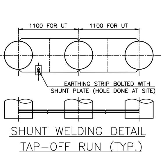
AL WELDED CONDUCTOR JOINT IN TAP-OFF RUN
