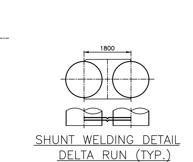
AL WELDED CONDUCTOR JOINT IN MAIN & DELTA RUN
