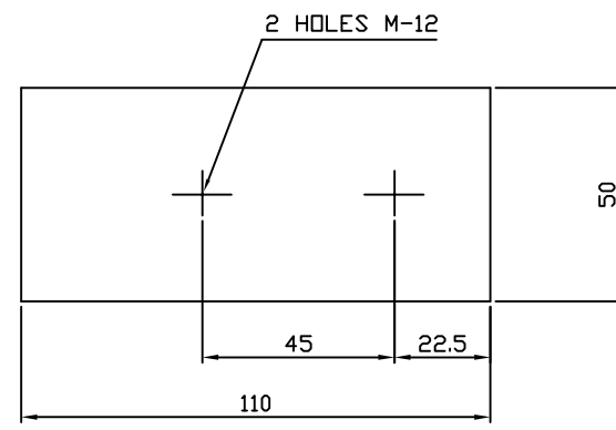
DETAIL - A (EARTHING DETAIL)
