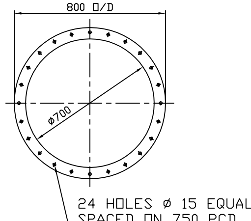
H.V. BUSDUCT (IPBD) FLANGE DETAIL DETAIL-C
