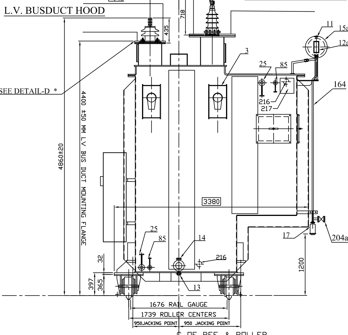
END VIEW
