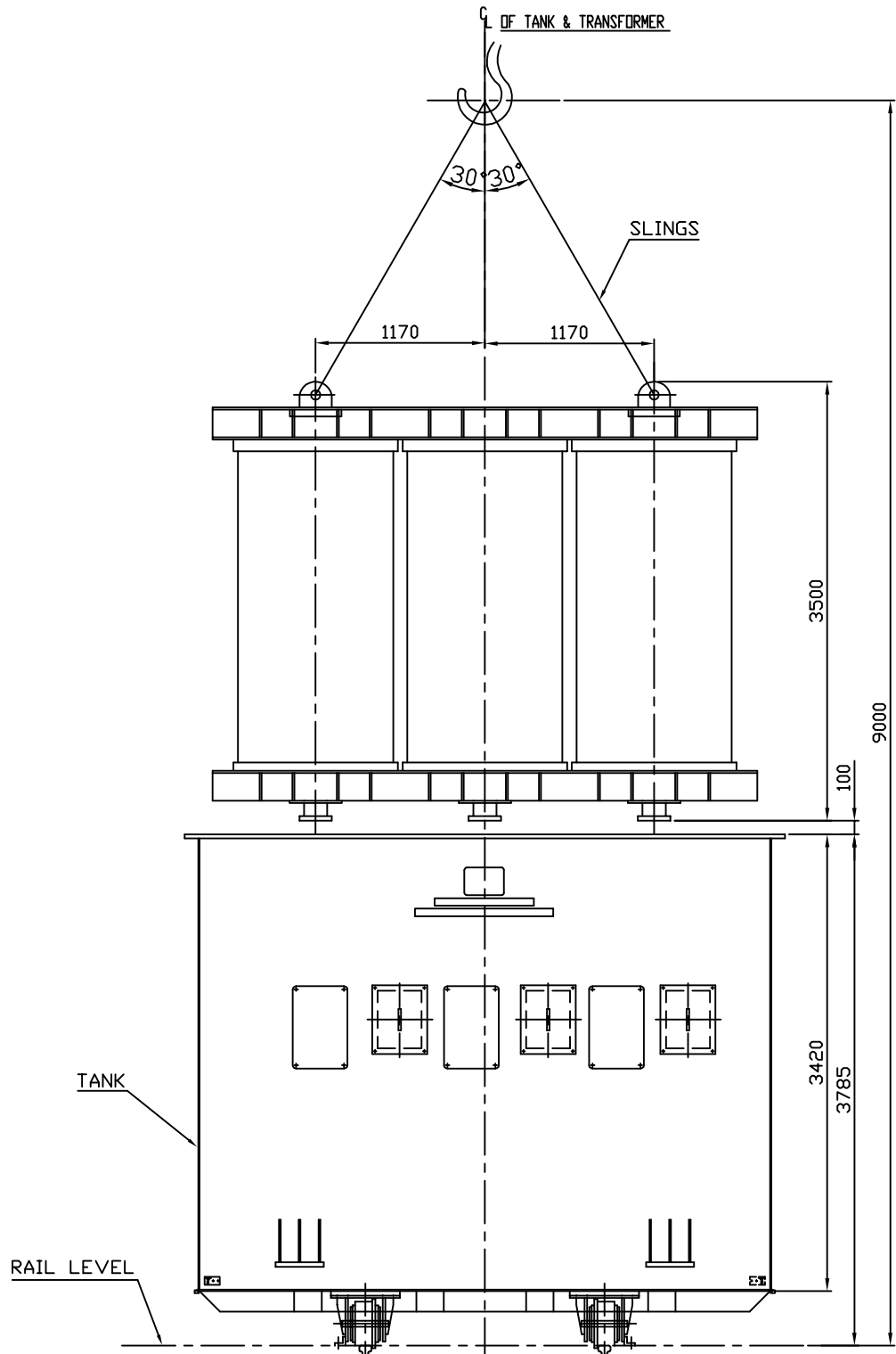
UNTANKING DETAIL
