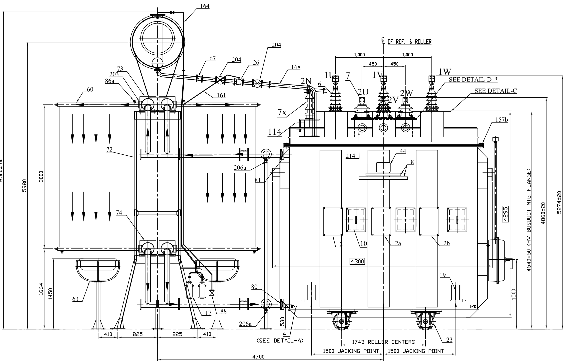
ELEVATION VIEW
