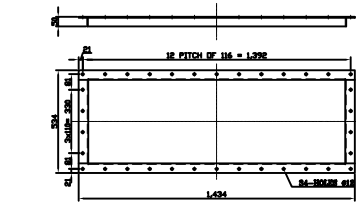
L.V. BUSDUCT (SPBD) FLANGE DETAIL DETAIL-D
