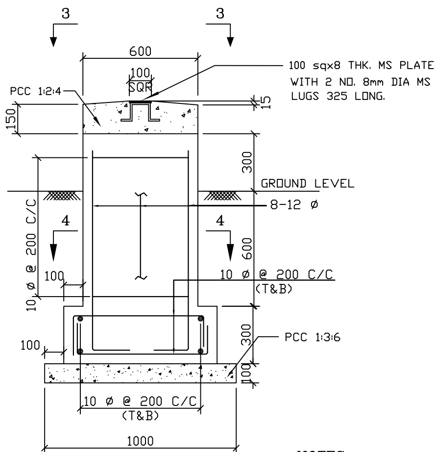
FIG. 2 GRID PILLAR/REFERENCE PILLAR
