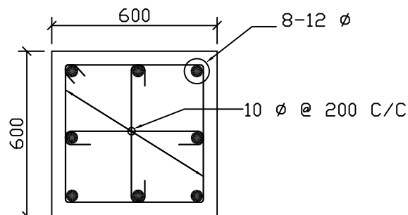
SECTION 4-4
