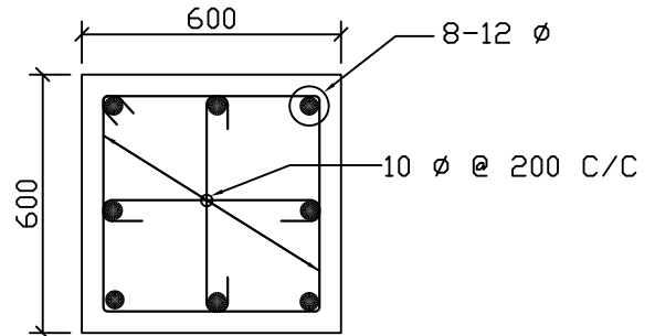
SECTION 2-2
