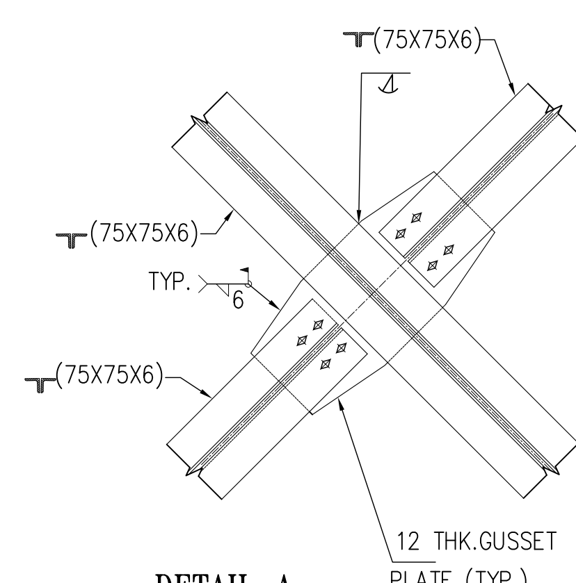
DETAIL-A
