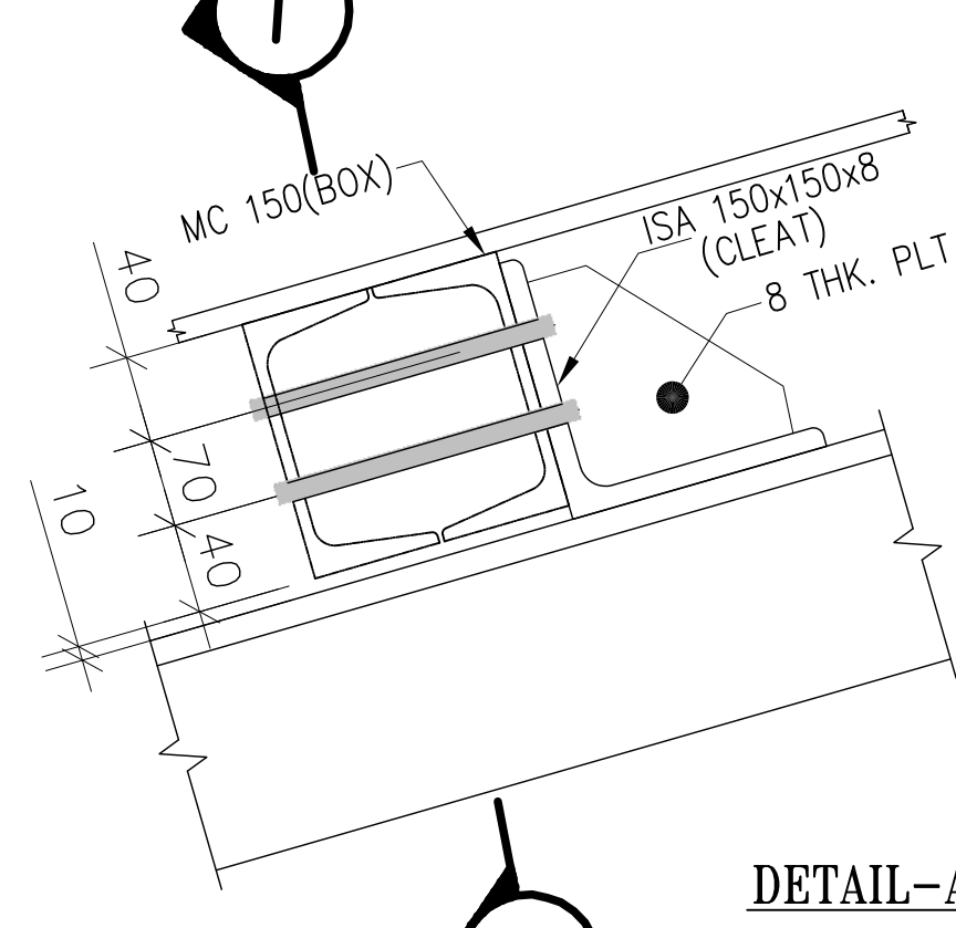
DETAIL-A
