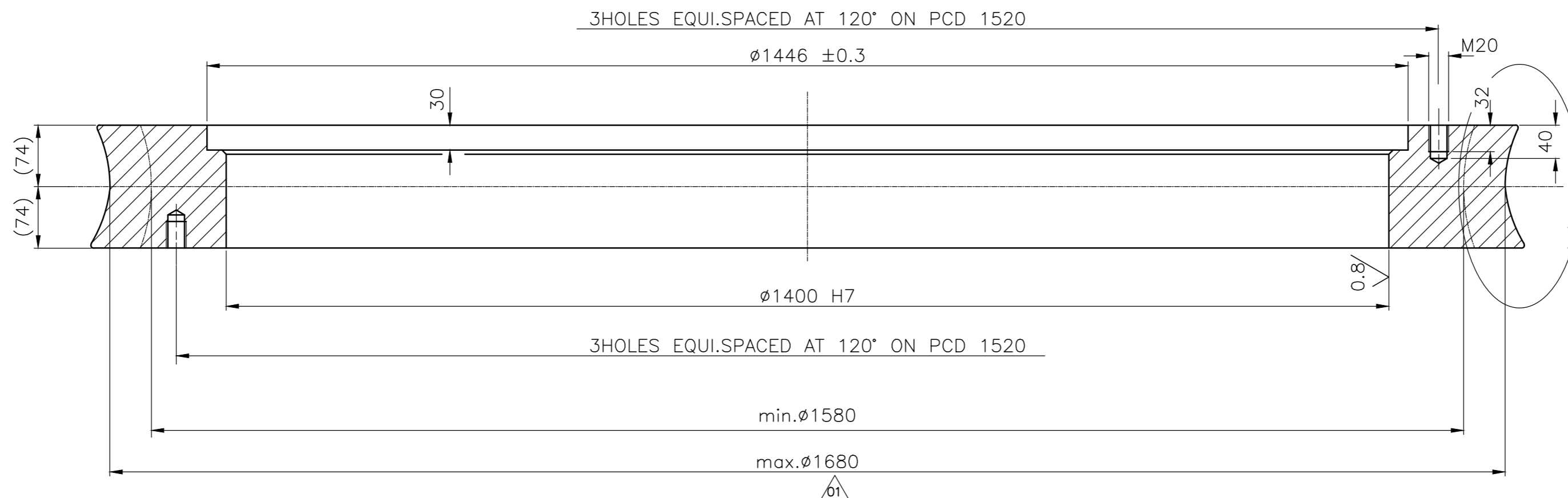
DETAIL-X
