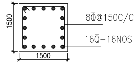
REINFORCEMENT DETAIL OF PEDESTAL
