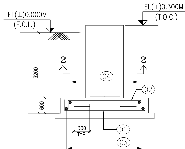
SECTION 1-1
