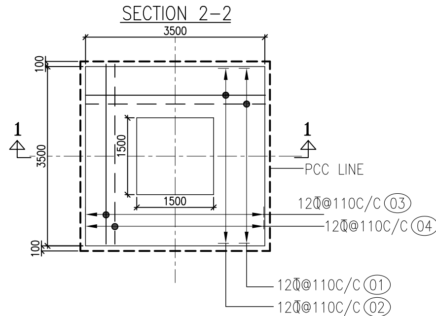
REINFORCEMENT DETAIL OF FOUNDATION PAD
