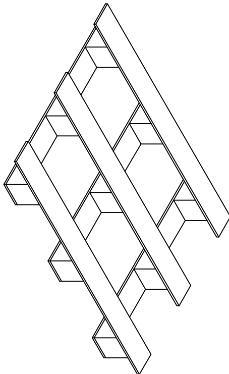
ISO-METRIC VIEW OF PALLET
