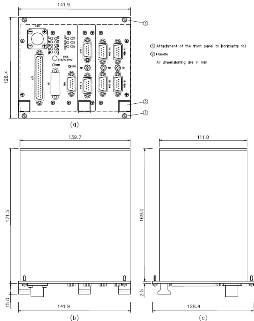
Fig.1- Dimensional details
