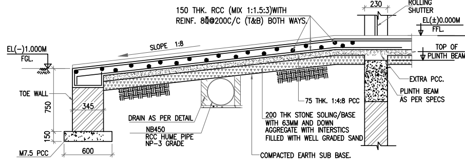
DETAIL OF RAMP
