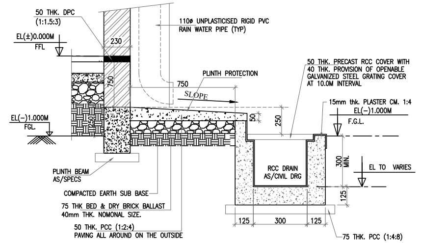
PLINTH PROTECTION ALONG BUILDING WITH DRAIN-TYPICAL
