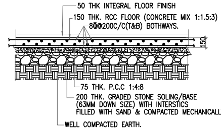
DETAIL OF GRADE SLAB
