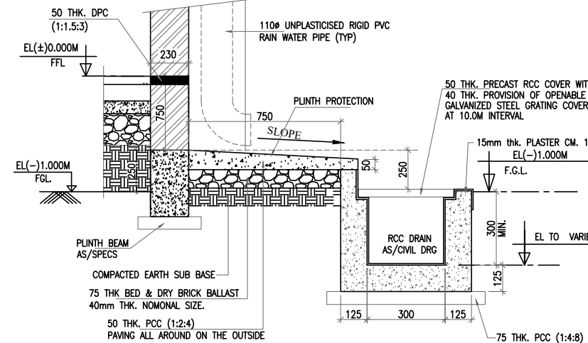
PLINTH PROTECTION ALONG BUILDING WITH DRAIN-TYPICAL
