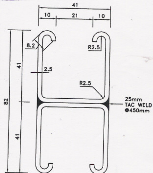
DOUBLE CHANNEL DCI
