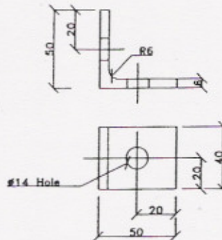
90° ANGLE FITTING LA1
