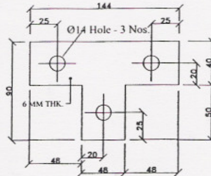
FLAT PLATE TEE FITTING PF1
