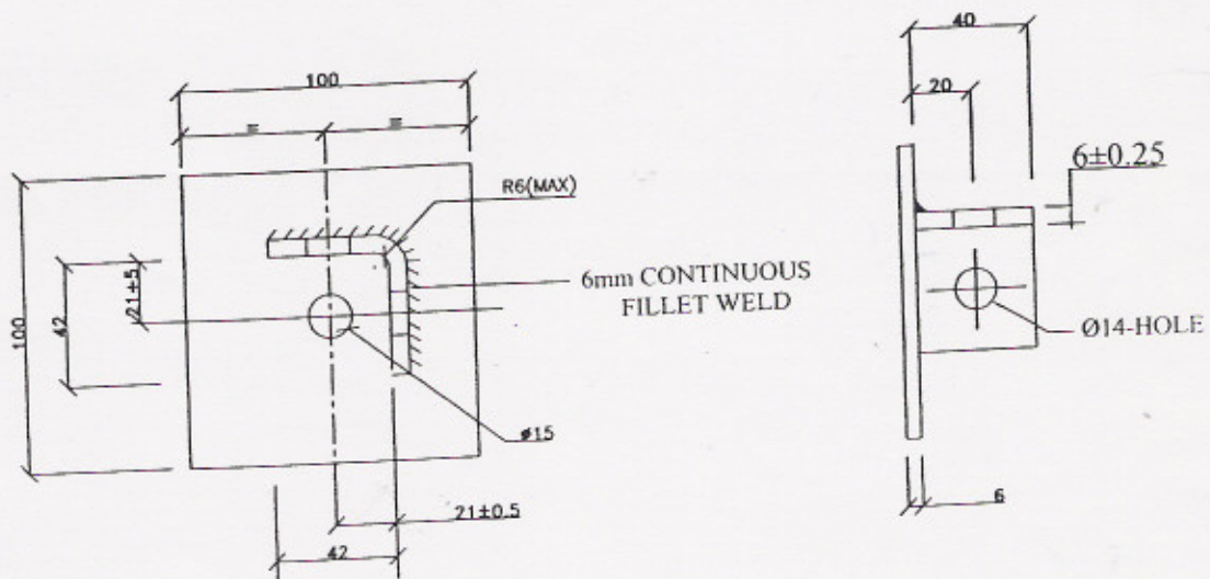
BASE PLATE FOR SINGLE CHANNEL BPI
