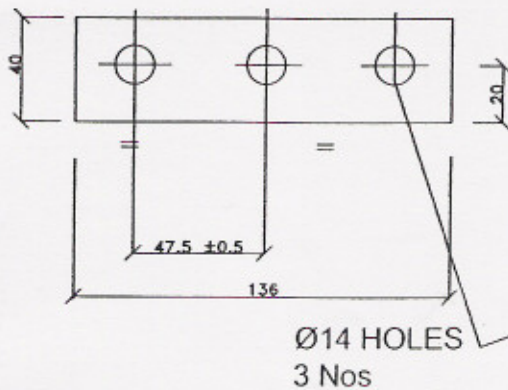
CLAMP FOR SINGLE CHANNEL CC1
