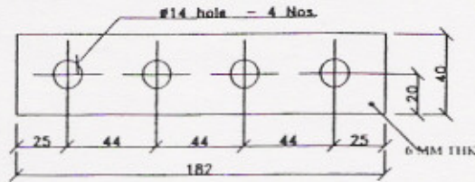
FLAT PLATE STRAIGHT FITTING PF2
