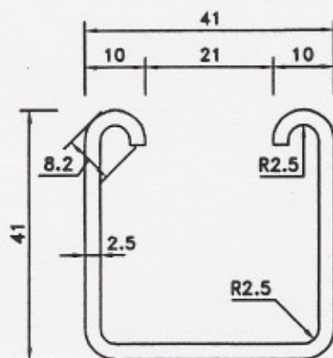
SINGLE CHANNEL SCI
