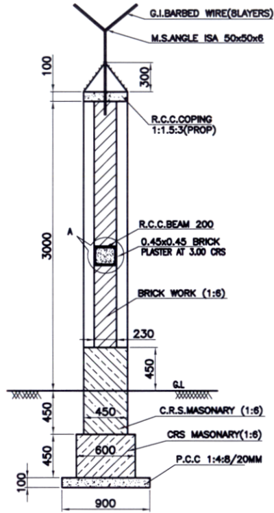
CROSS SECTION
