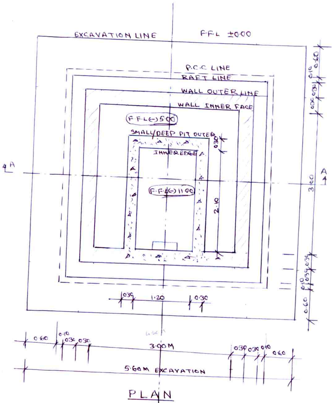
STACK PIT FOUNDATION (9FA)
