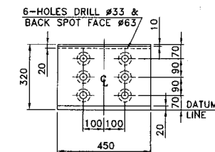
VIEW AS ARROW-C
