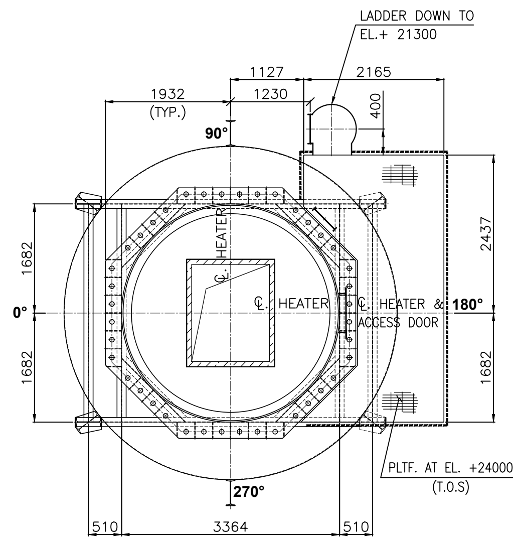
SECTION H-H
