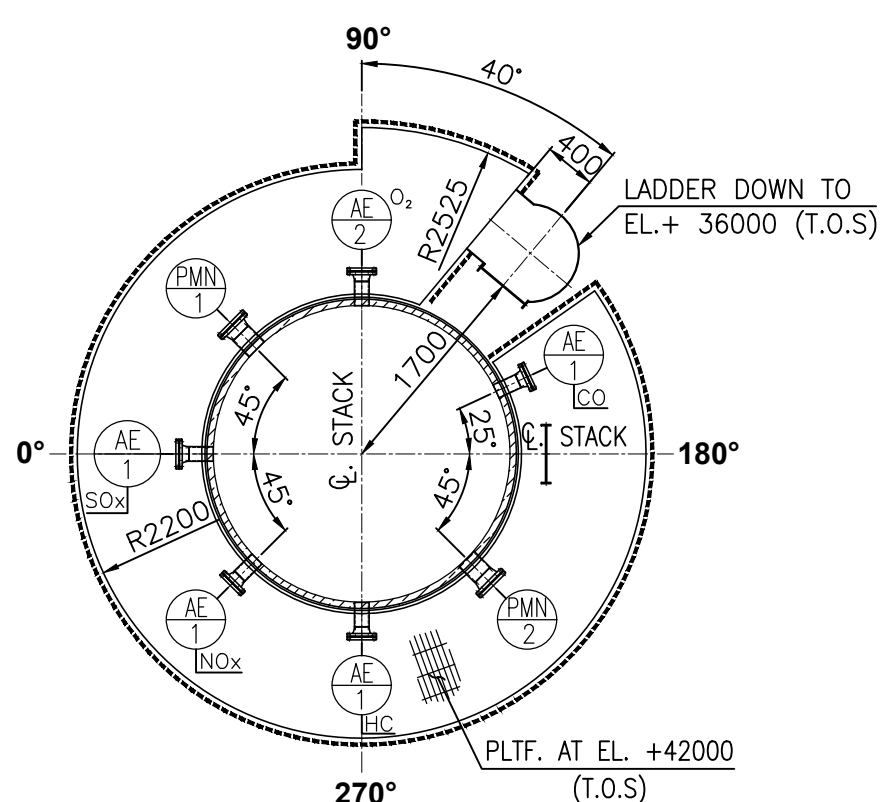
SECTION L-L
