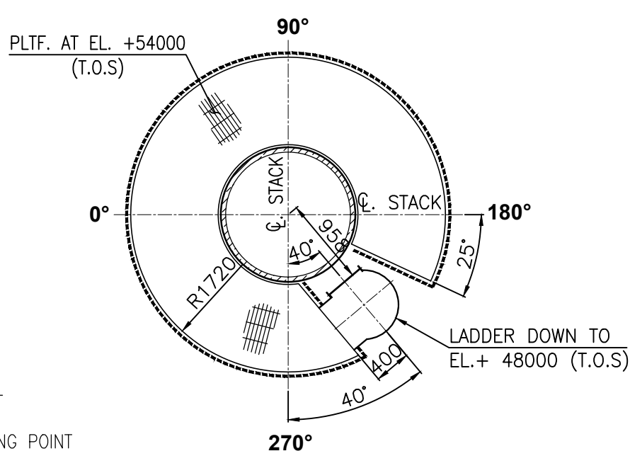
SECTION N-N
