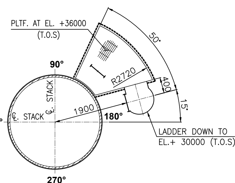
SECTION K-K
