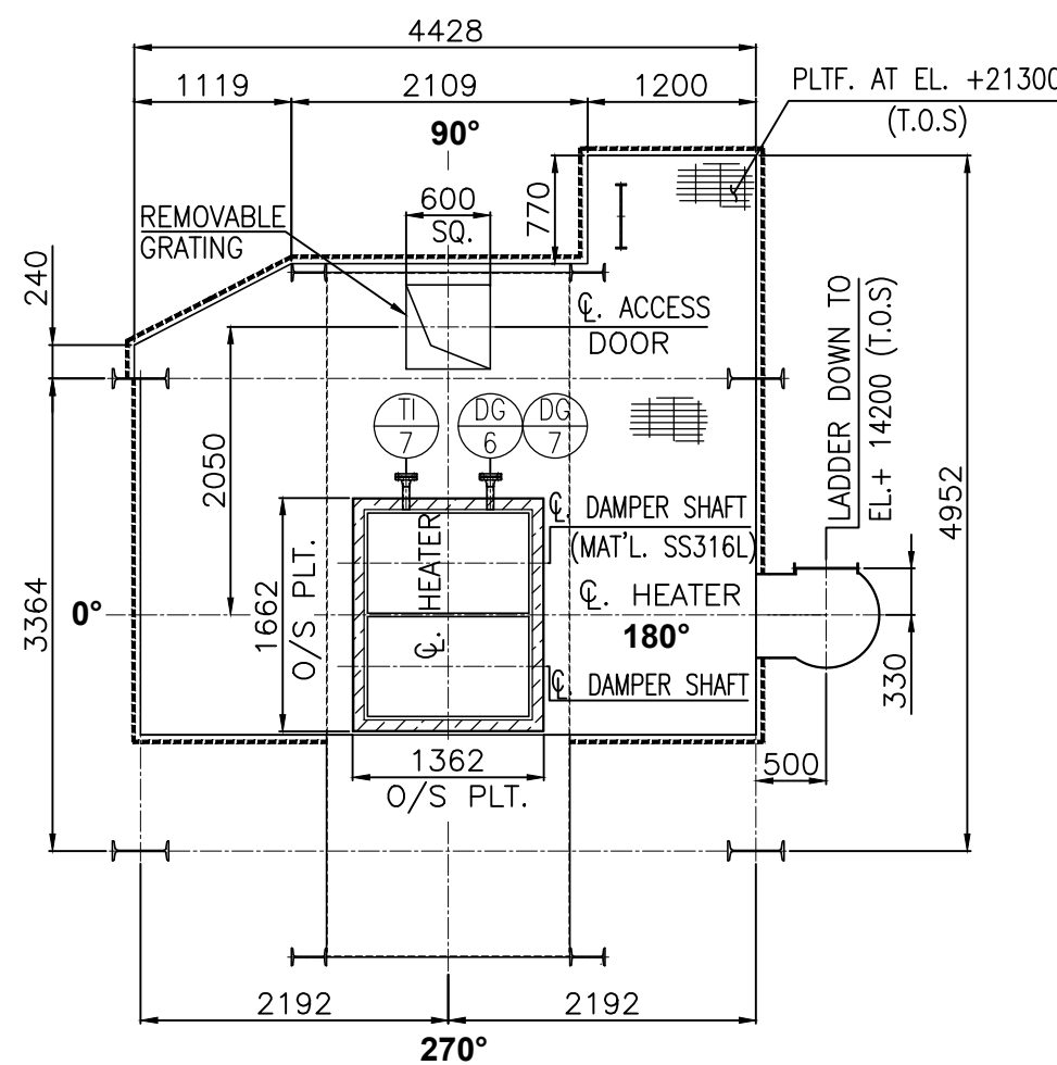
SECTION G-G
