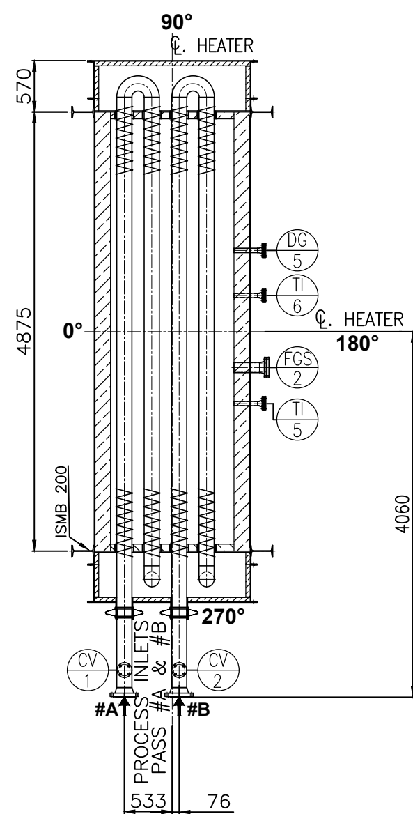
SECTION F-F
