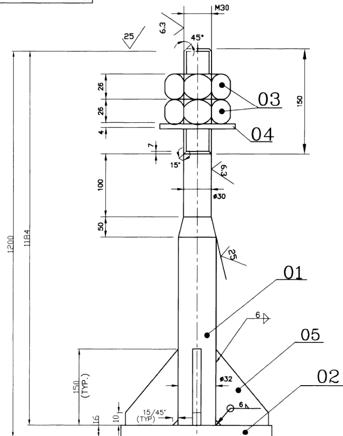
VIEW - "A"
