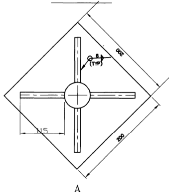
VIEW - "A"
