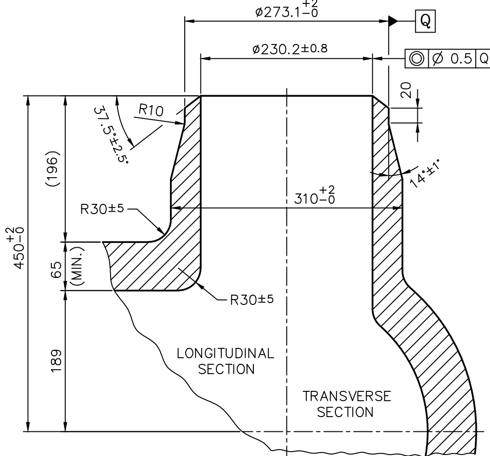
SECTION-BB (250 NB) (1:5)
