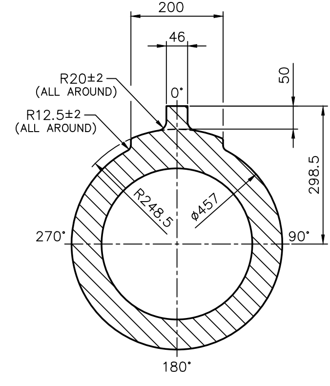
SECTION-DD (VIEW WITHOUT LARGE SIZE NOZZLE DETAILS) (1:8)
