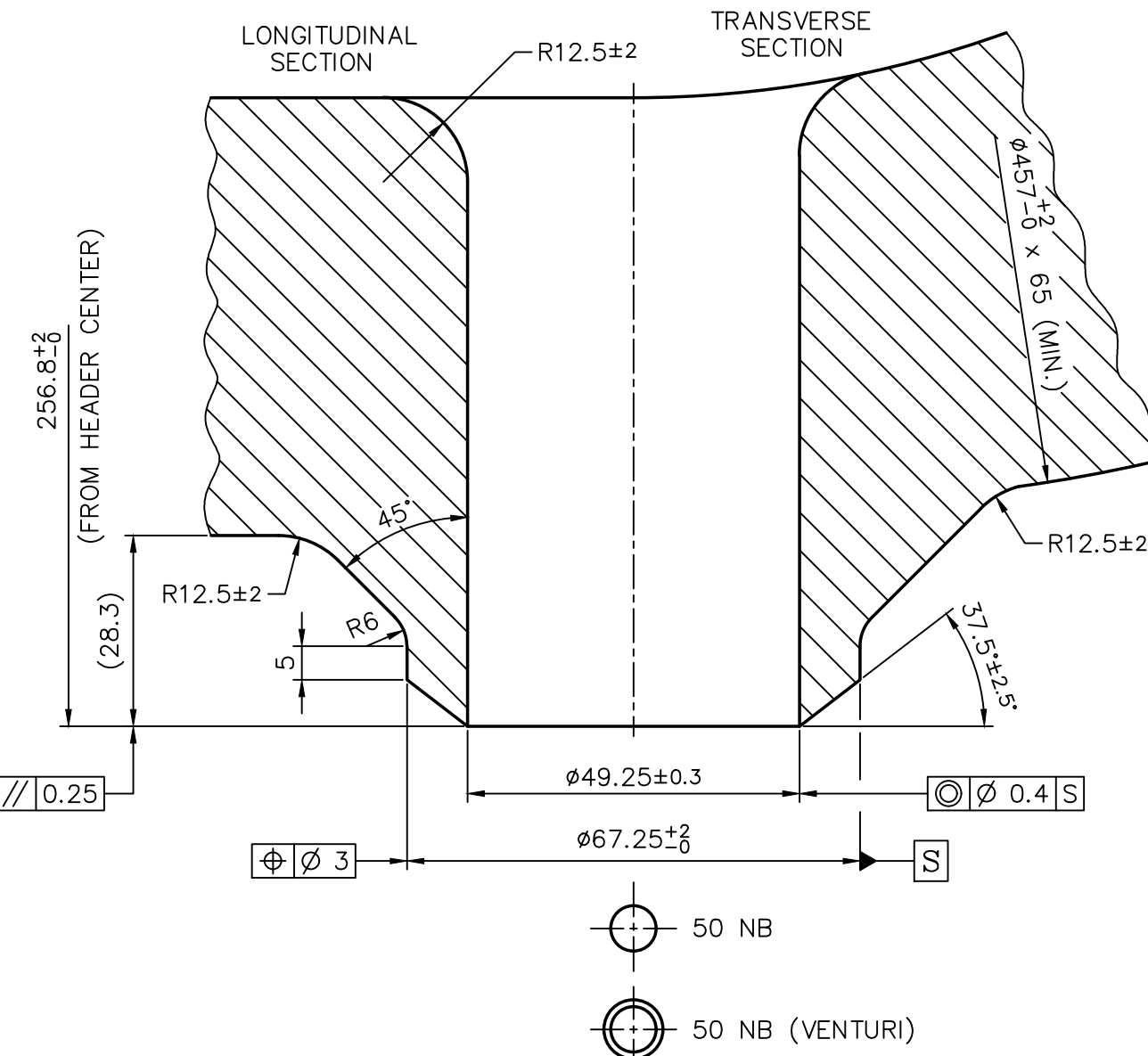
50 NB NOZZLE DETAILS (1:1)
