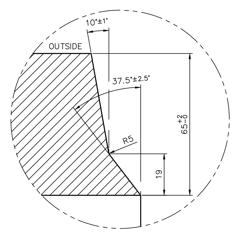
DETAIL-1 (1:1)
