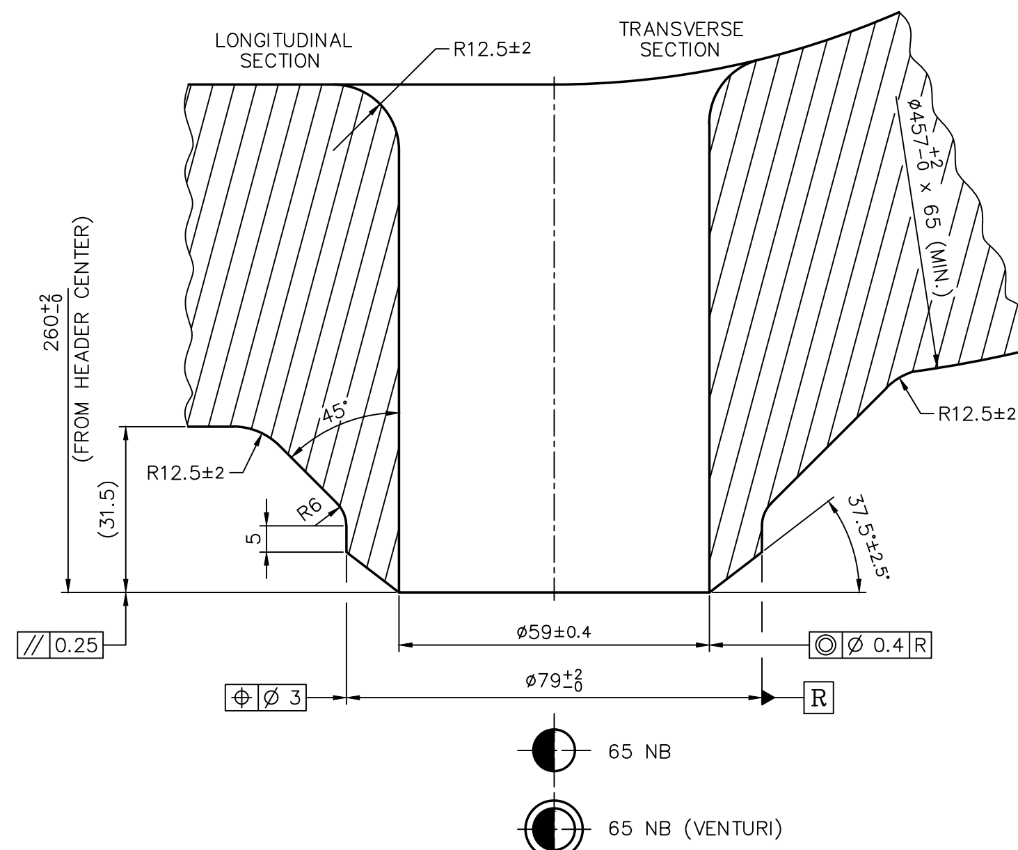
65 NB NOZZLE DETAILS (1:1)
