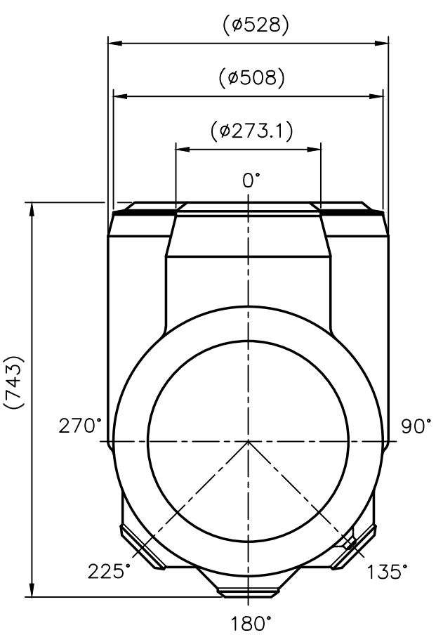
VIEW-X (1:10)
