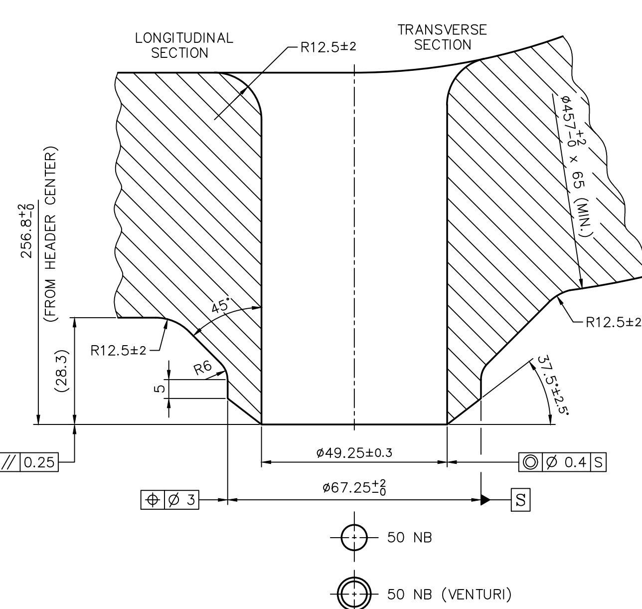
50 NB NOZZLE DETAILS (1:1)
