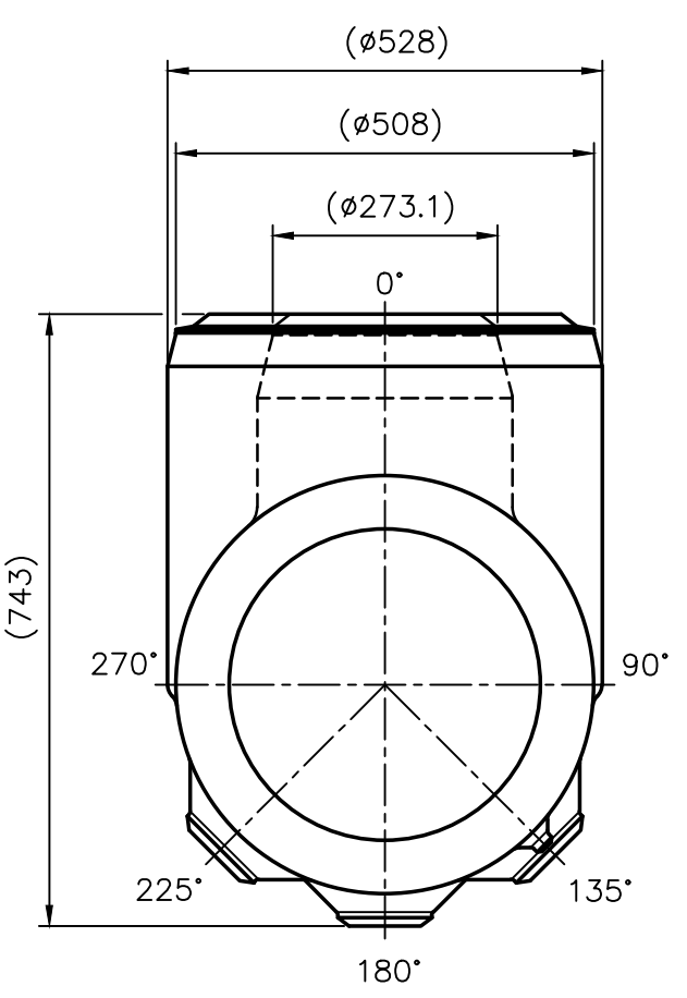
VIEW-X (1:10)
