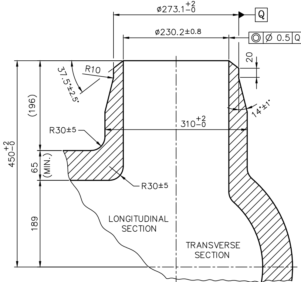
SECTION-BB (250 NB) (1:5)
