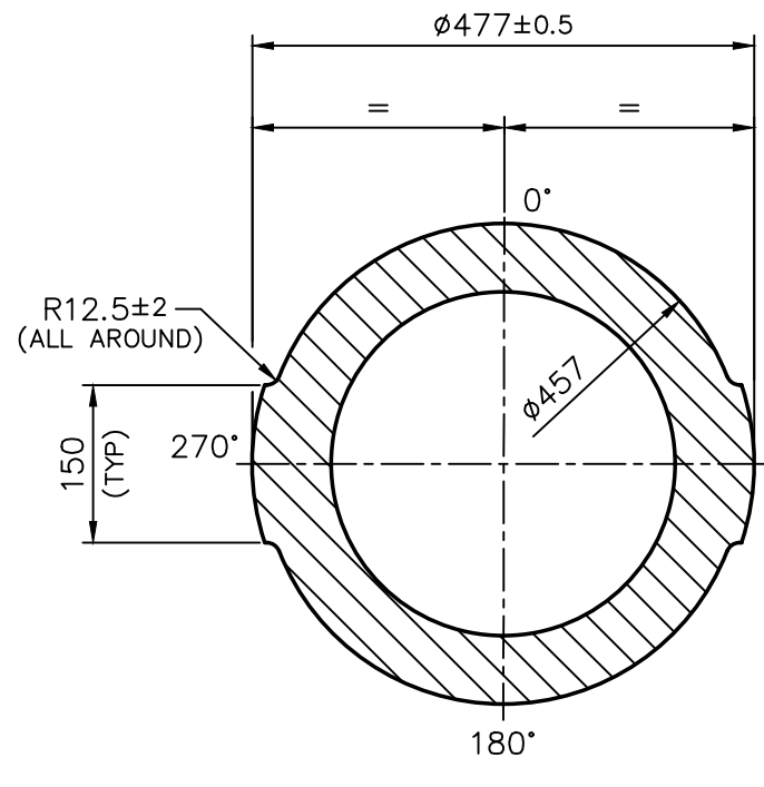
SECTION-CC (VIEW WITHOUT LARGE SIZE NOZZLE DETAILS) (1:8)
