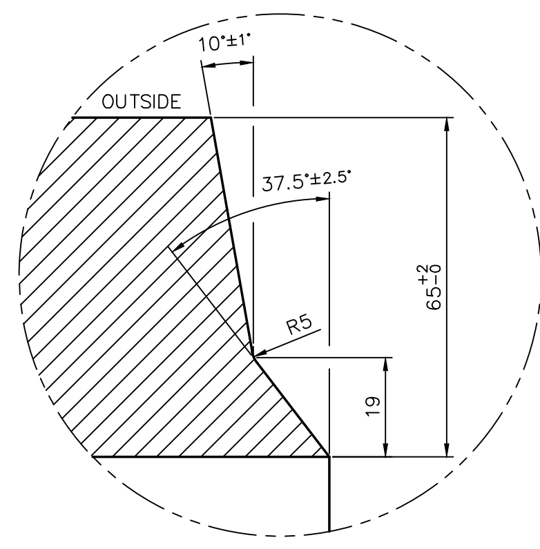
DETAIL-1 (1:1)
