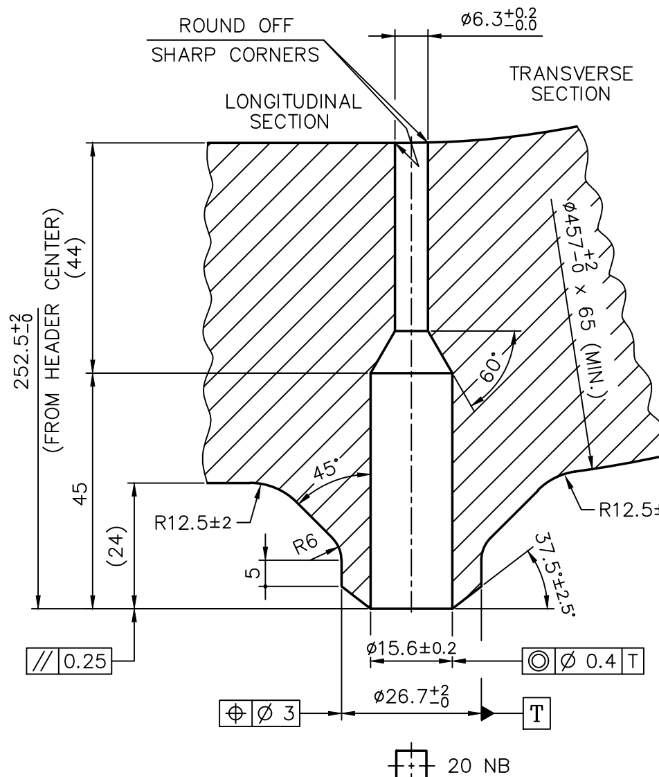
20 NB NOZZLE DETAILS (1:1)
