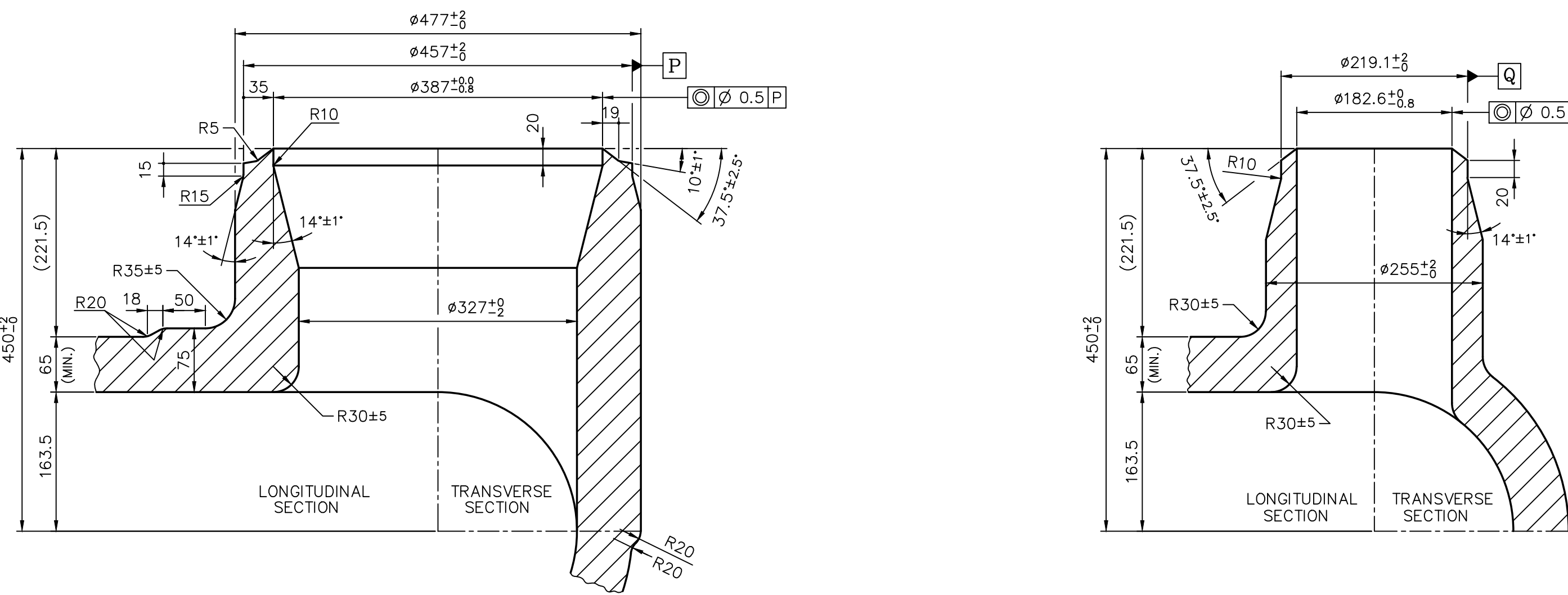
SECTION-AA (450 NB) (1:5)
