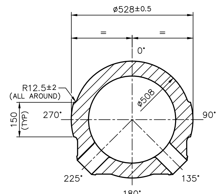
SECTION-CC (VIEW WITHOUT LARGE SIZE NOZZLE DETAILS) (1:10)
