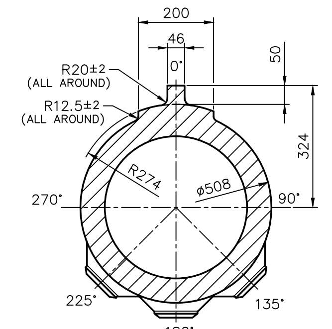
SECTION-DD (VIEW WITHOUT LARGE SIZE NOZZLE DETAILS) (1:10)
