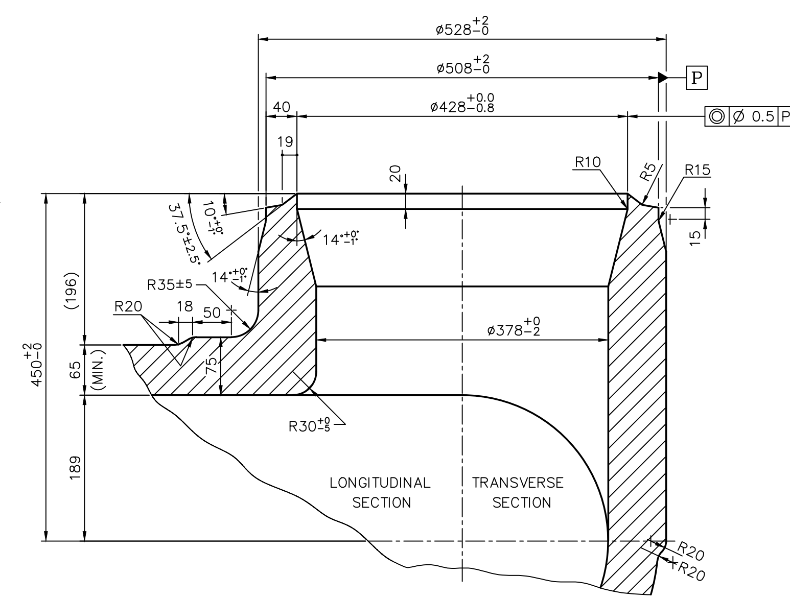
SECTION-AA (500 NB) (1:5)
