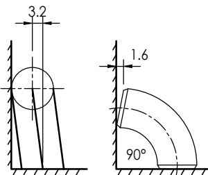
OFF-SQUARE TOLERANCES
