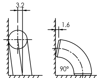
OFF-SQUARE TOLERANCES
