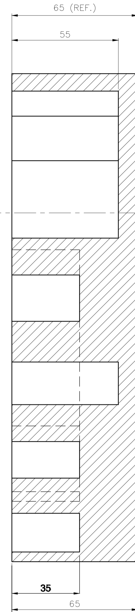
SECTION C-C
