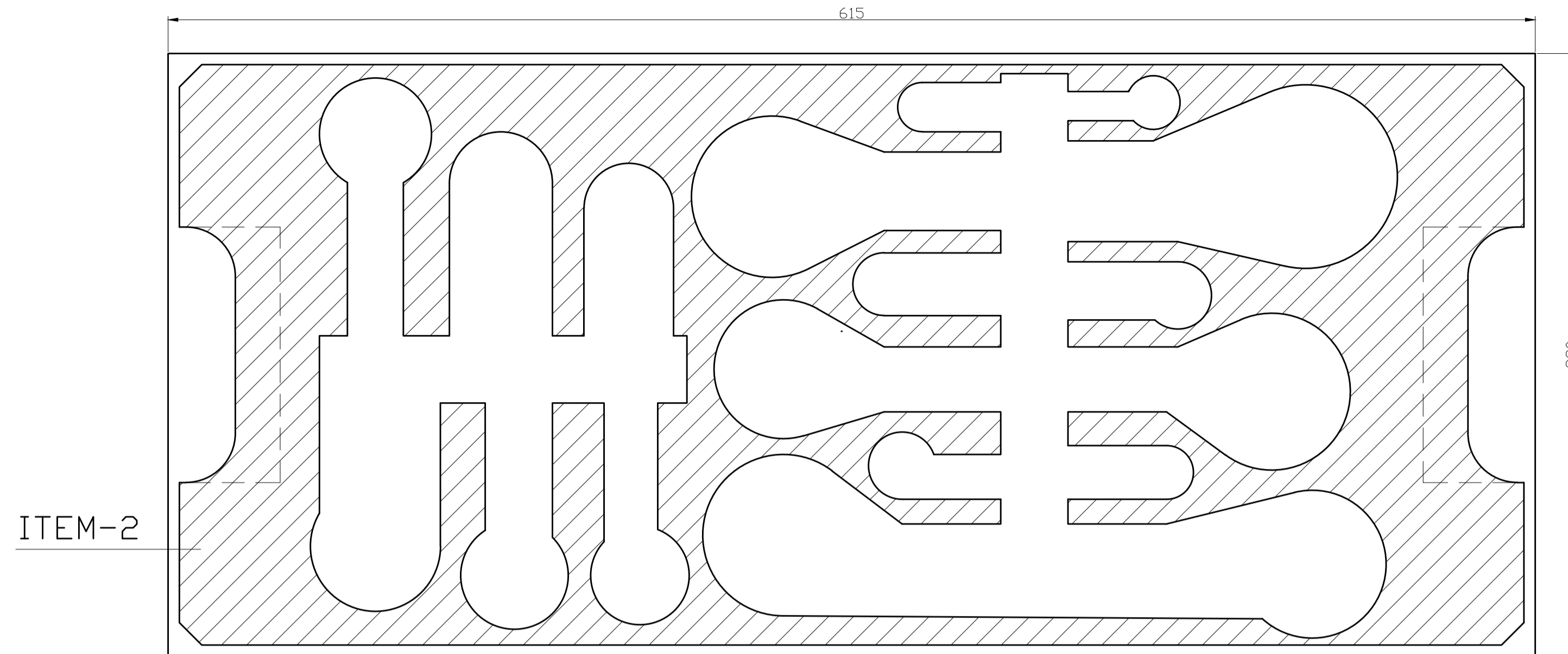
SECTION P-P
