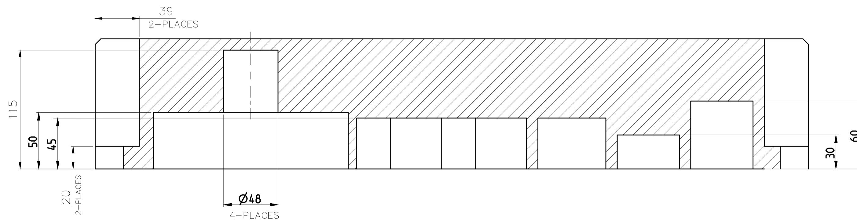
SECTION C-C
