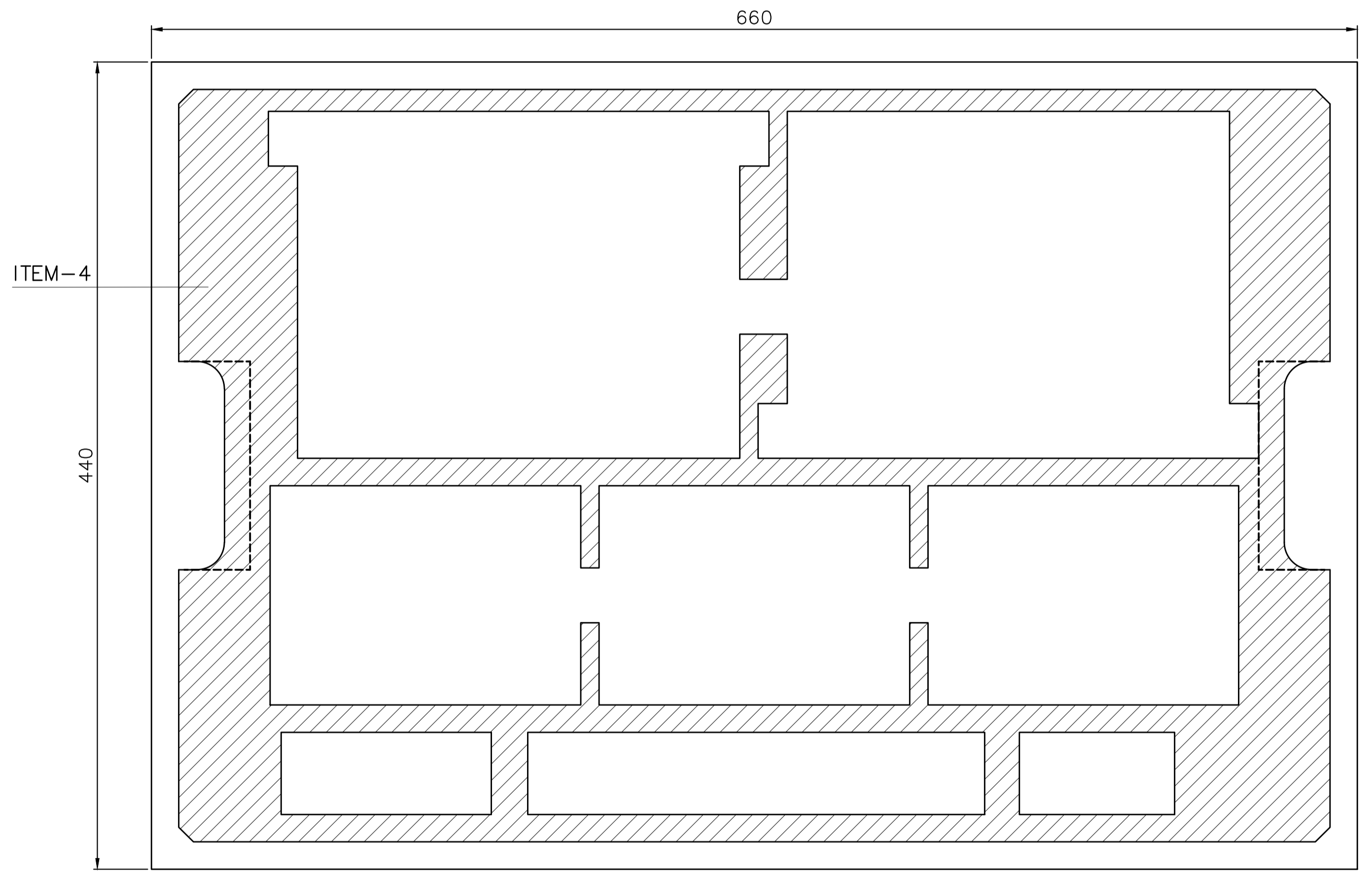
SECTION R-R
