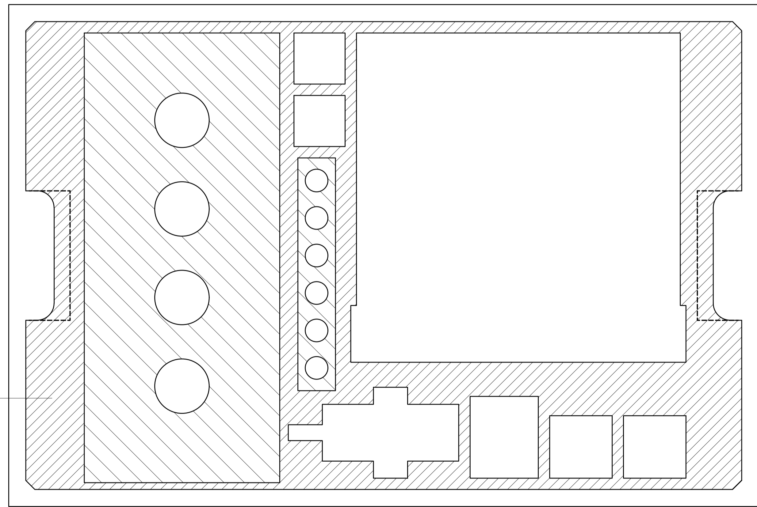
SECTION Q-Q
