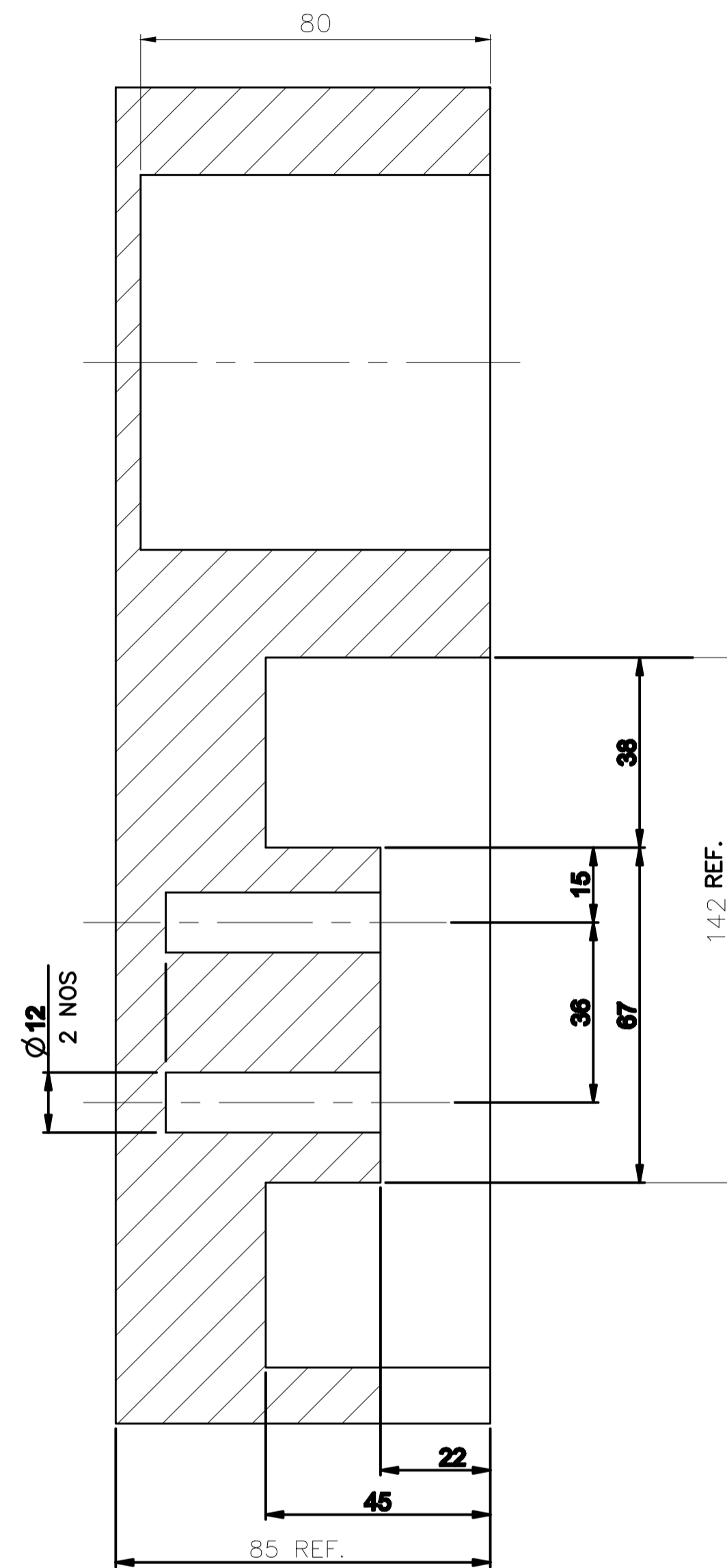
C-C (FROM SH- 3)
