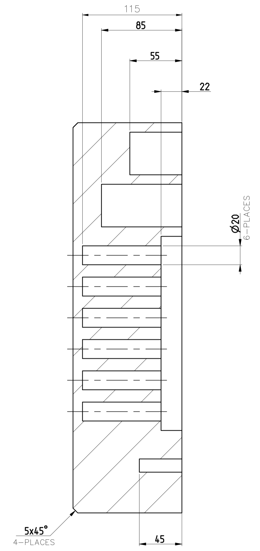
SECTION B-B
