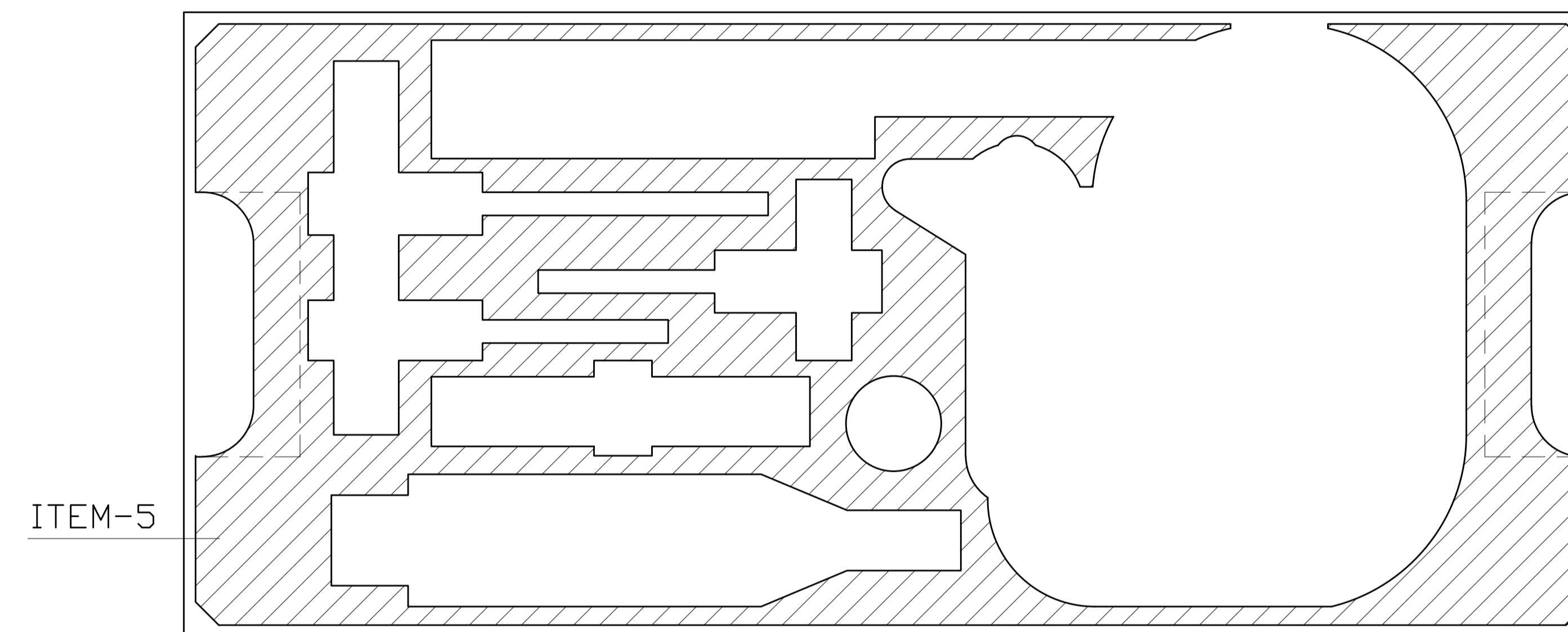
SECTION S-S
