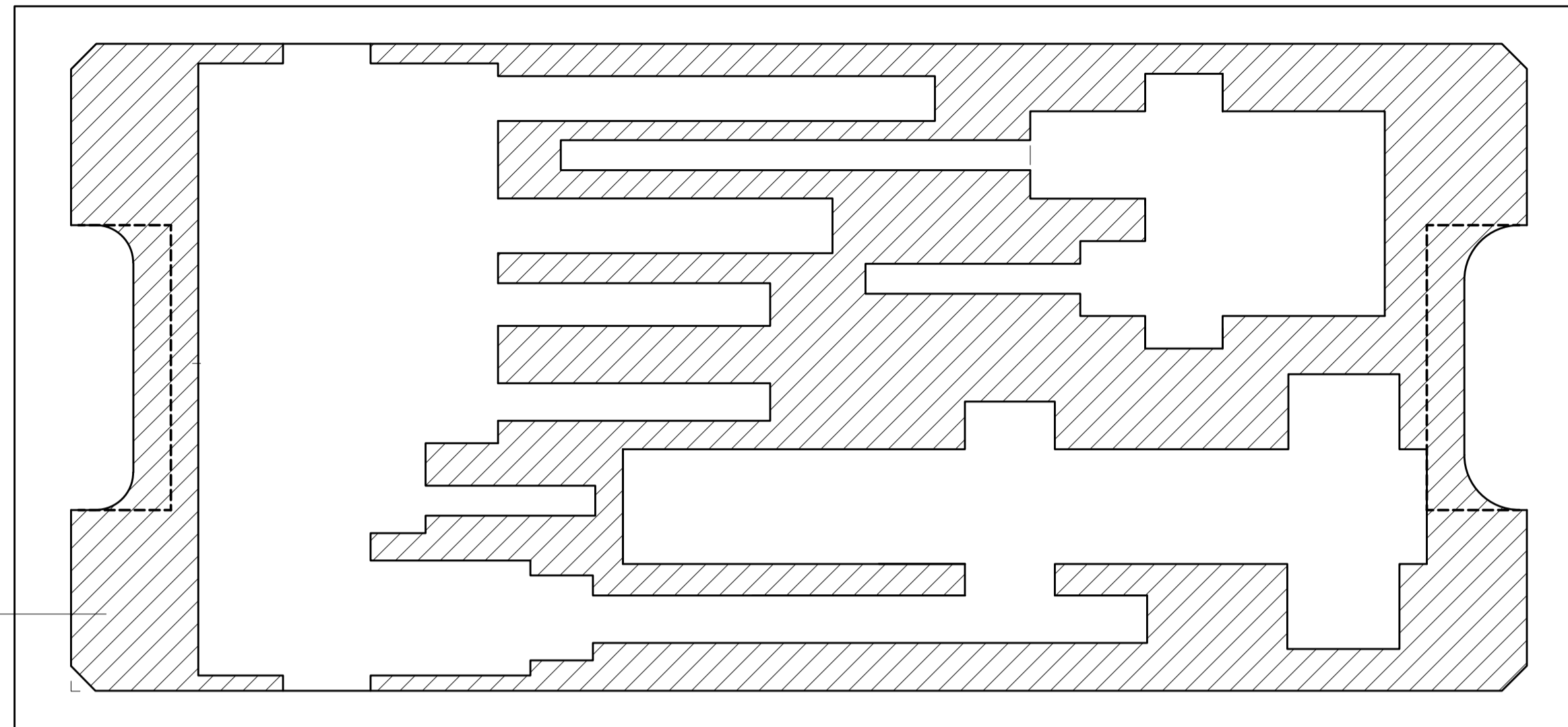
SECTION P-P
