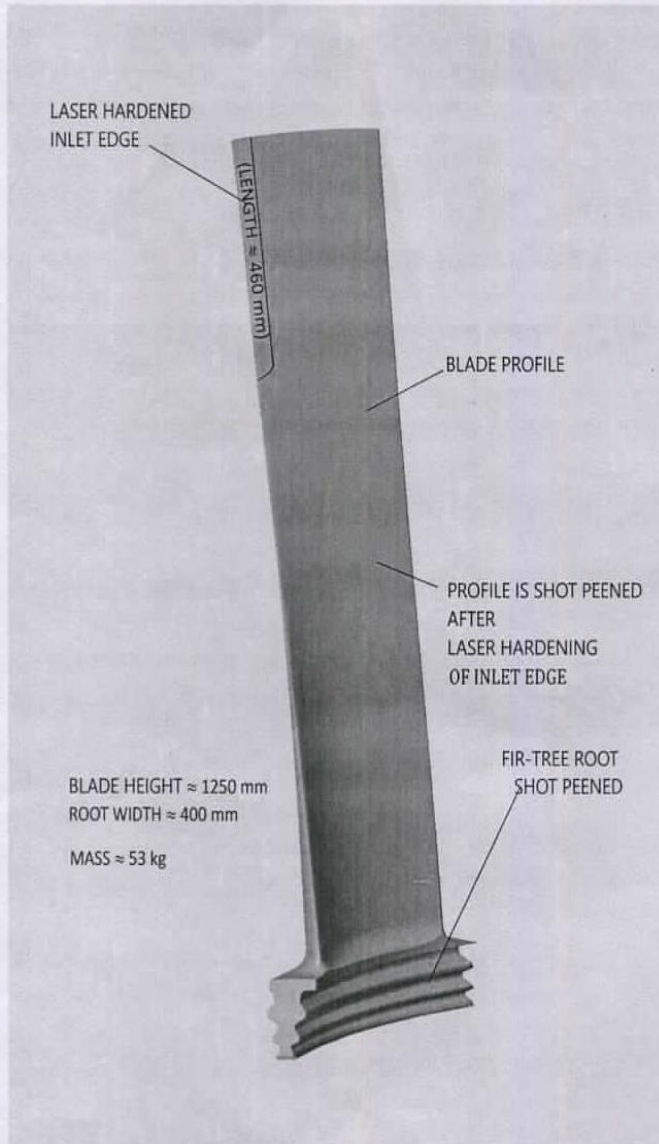
Figure 1: Blade details for reference
