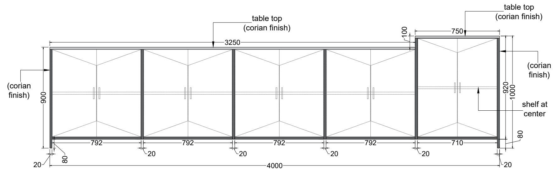
BACK ELEVATION
