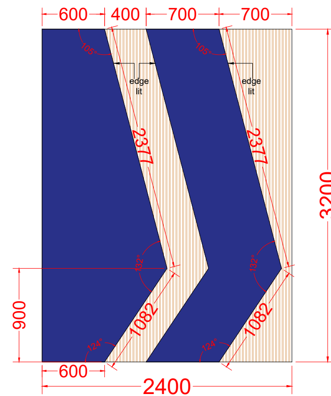
RECEPTION RIGHT SIDE WALL
