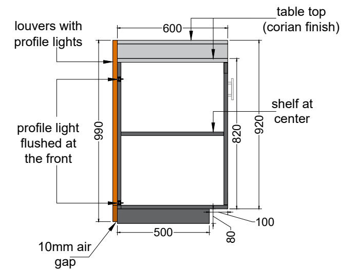
SECTIONAL SIDE ELEVATION
