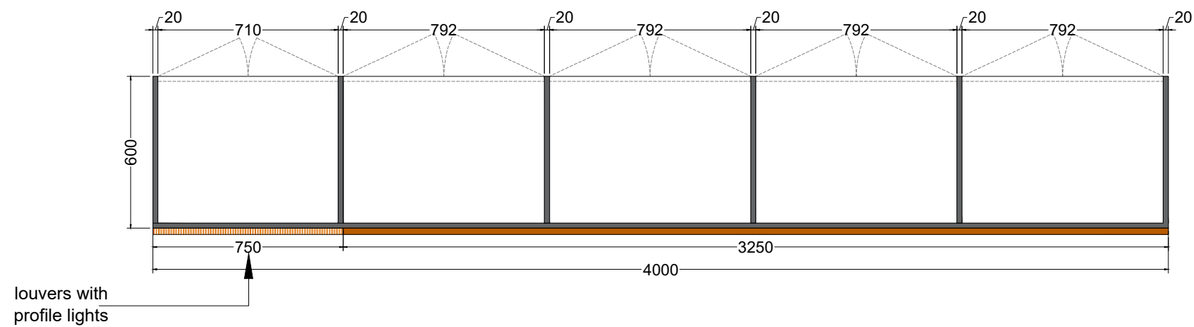
SECTIONAL PLAN
