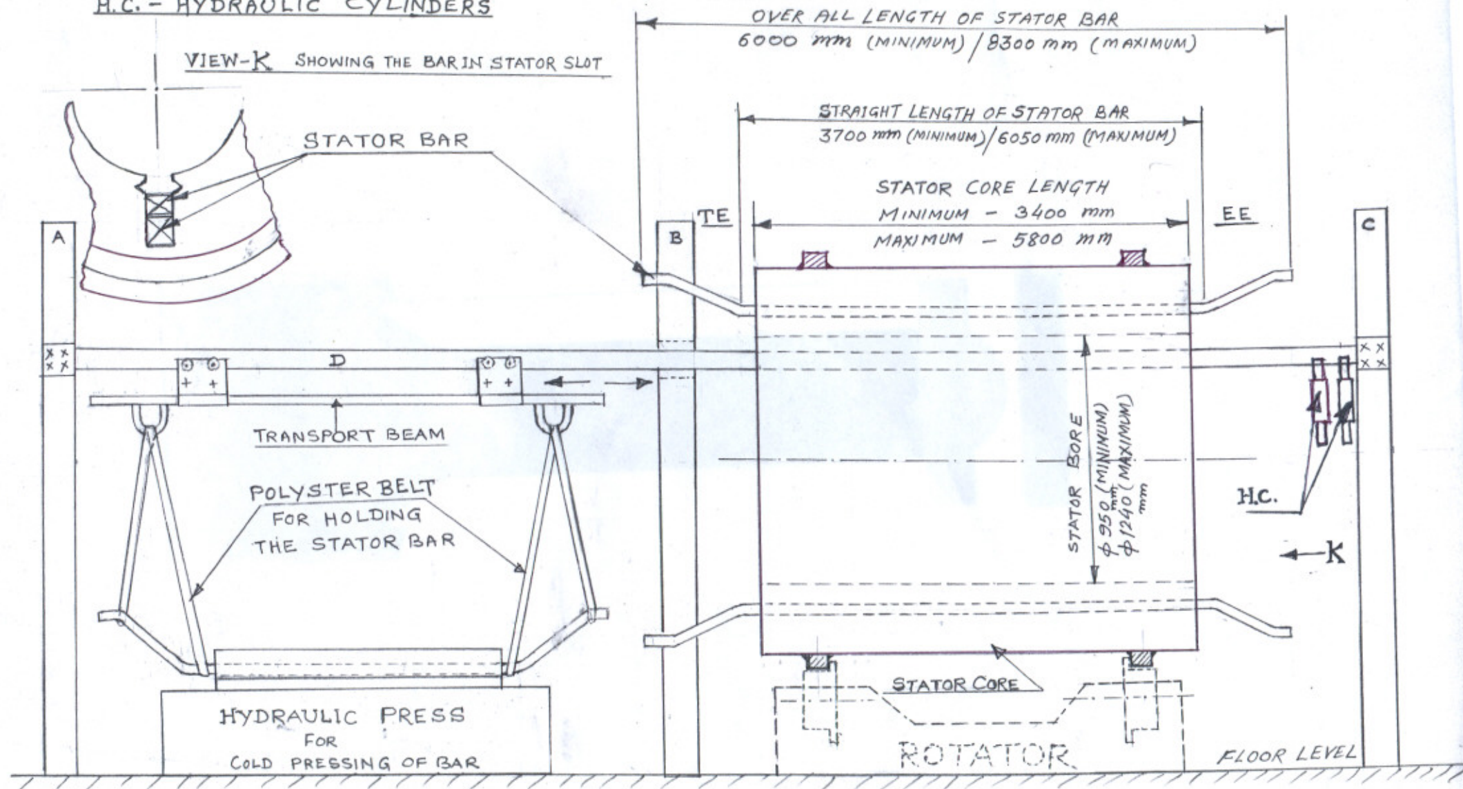
SCHEMATIC ARRANGEMENT OF FACILITY FOR BAR TRANSPORTATION AND INSERTION
