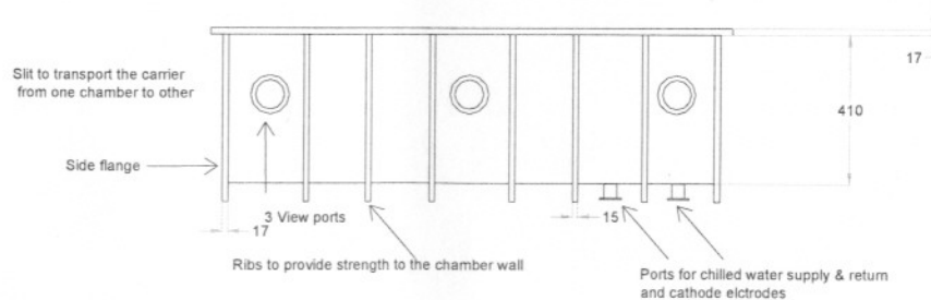
Front view without lid
