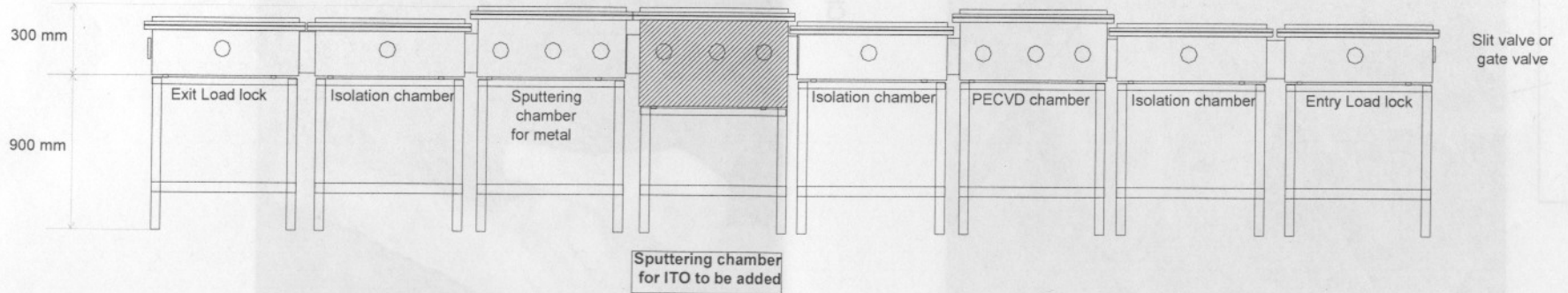
Proposed Modified Set of Vacuum Chambers
