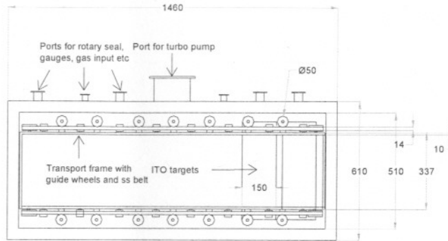
Top view without lid
