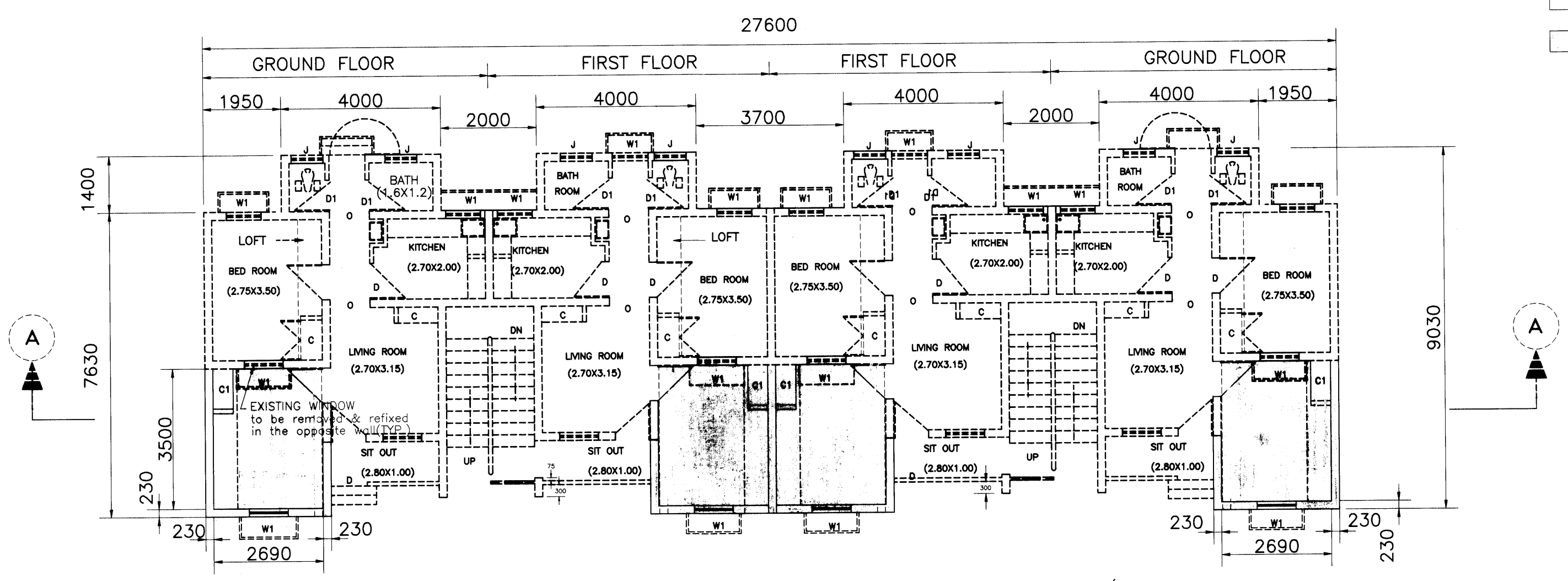
Plan of one block of eight houses Half Ground Floor & Half First Floor PLAN
