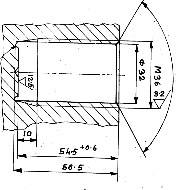
SECTION C-C
