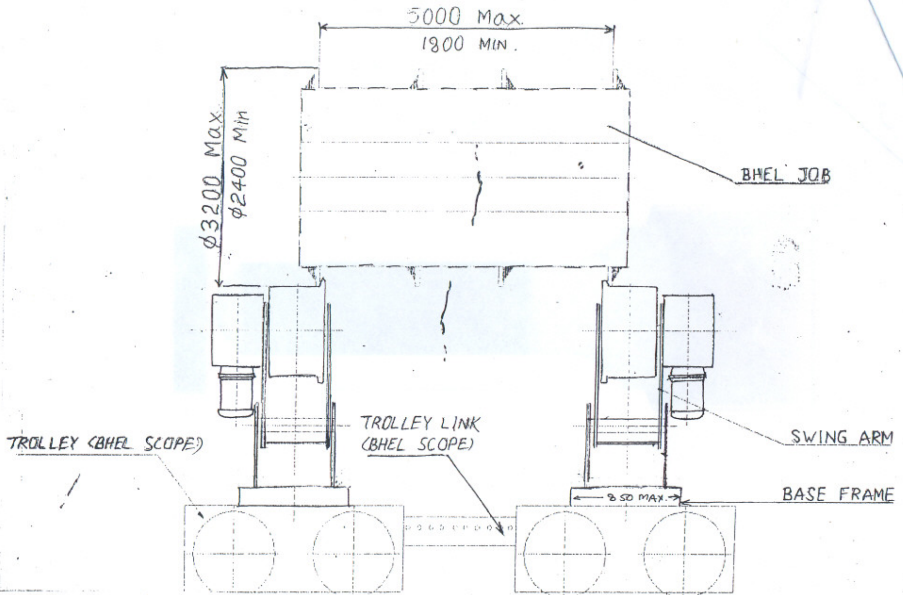
Schematic arrangement for mounting of wound stator core on rotator trolley
