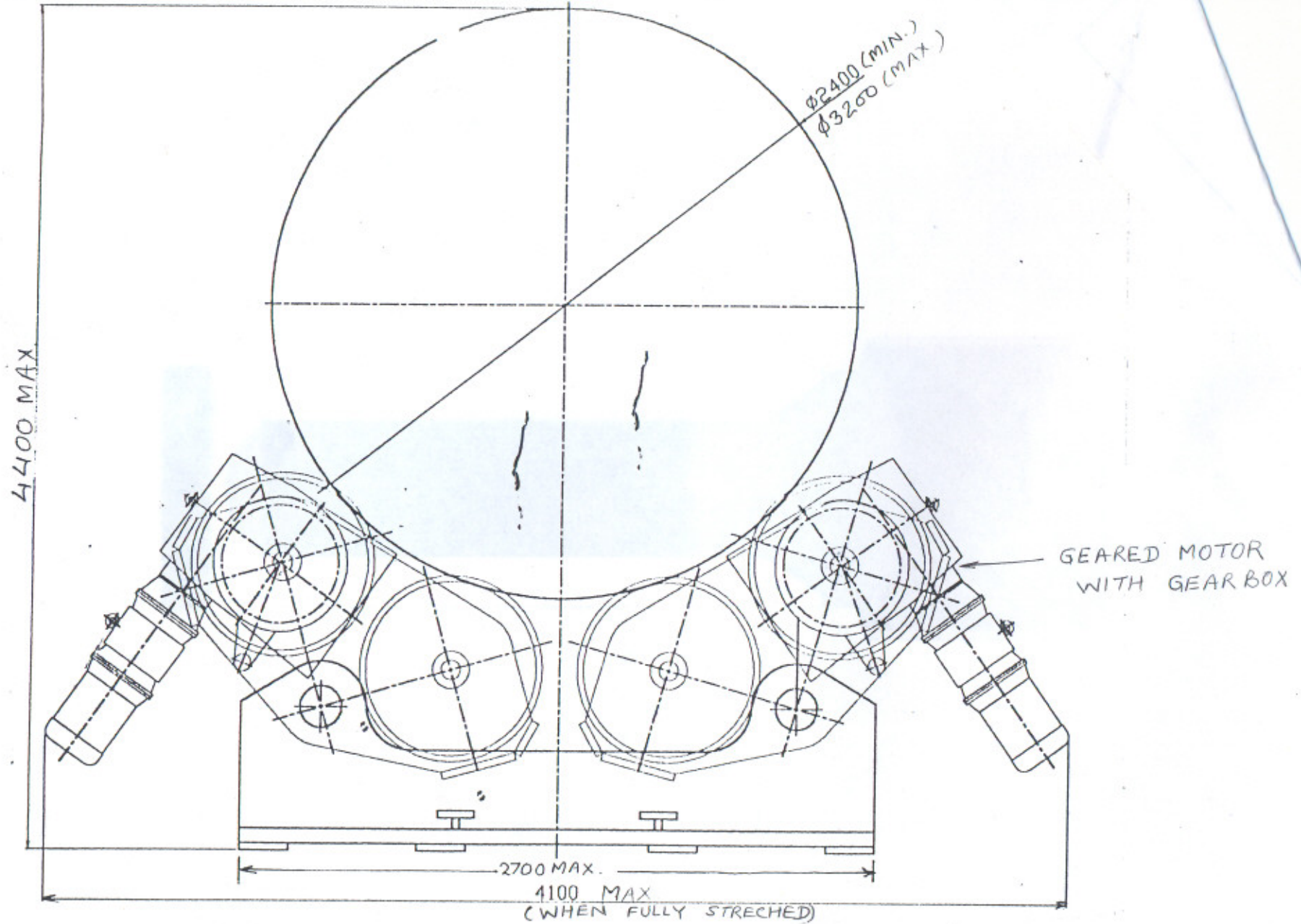
GENERAL LAYOUT OF 250 TONS CAPACITY SELF-ALLIGNED FLAME PROOF ROTATORS
