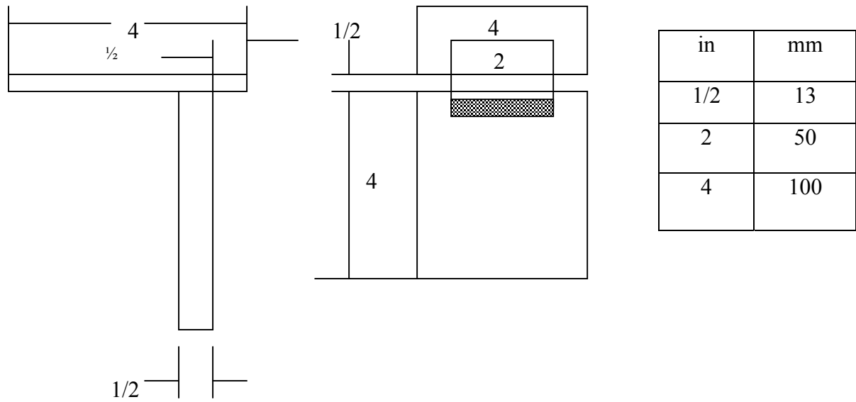
Fig 1 – Fillet Weld Break specimen
