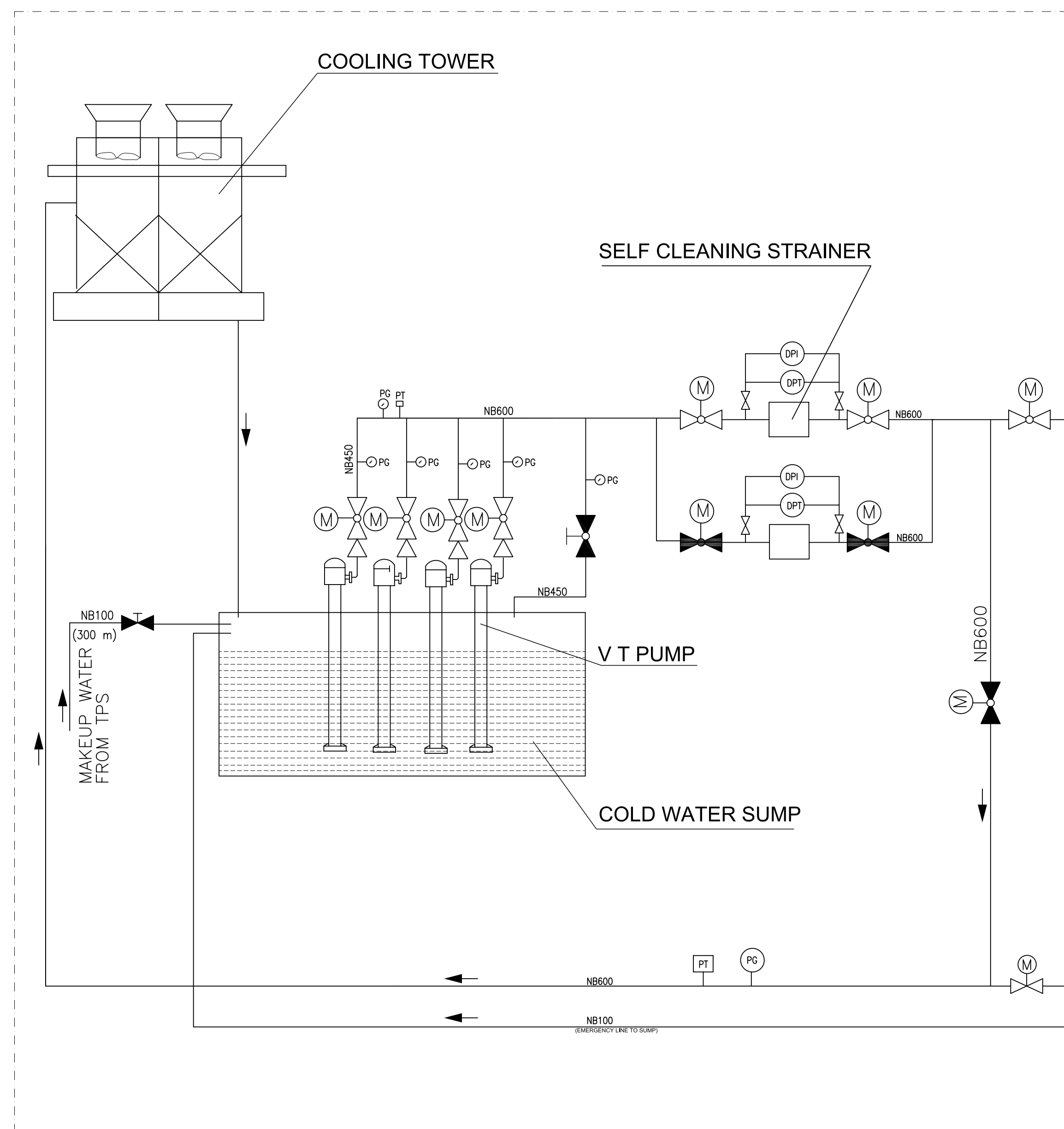
COOLING TOWER & PUMPHOUSE NEW PLANT
