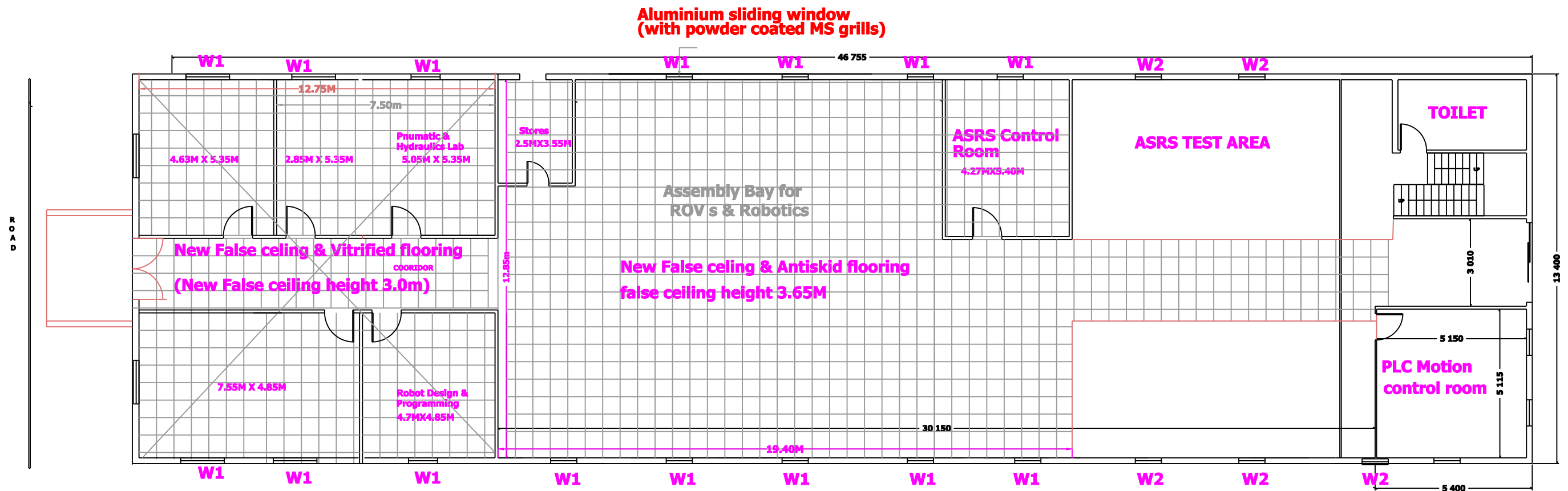
TDL GROUND FLOOR PLAN WITH Revised Partitions ,Flooring and Armstrong False ceiling
