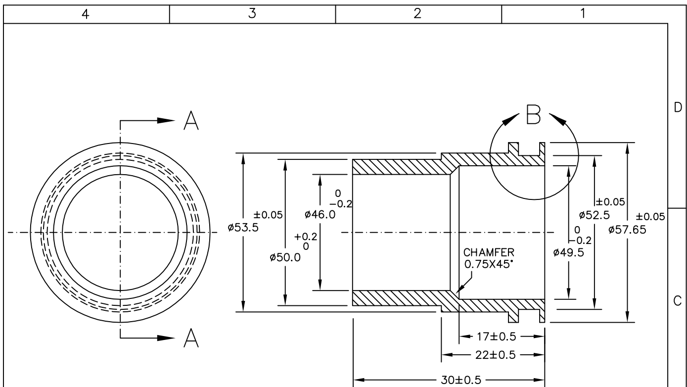
SECTION - AA
