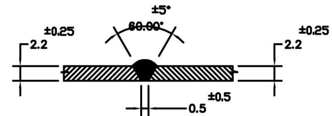
DETAILS OF L-SEAM WELD JOINTS A1, A2
