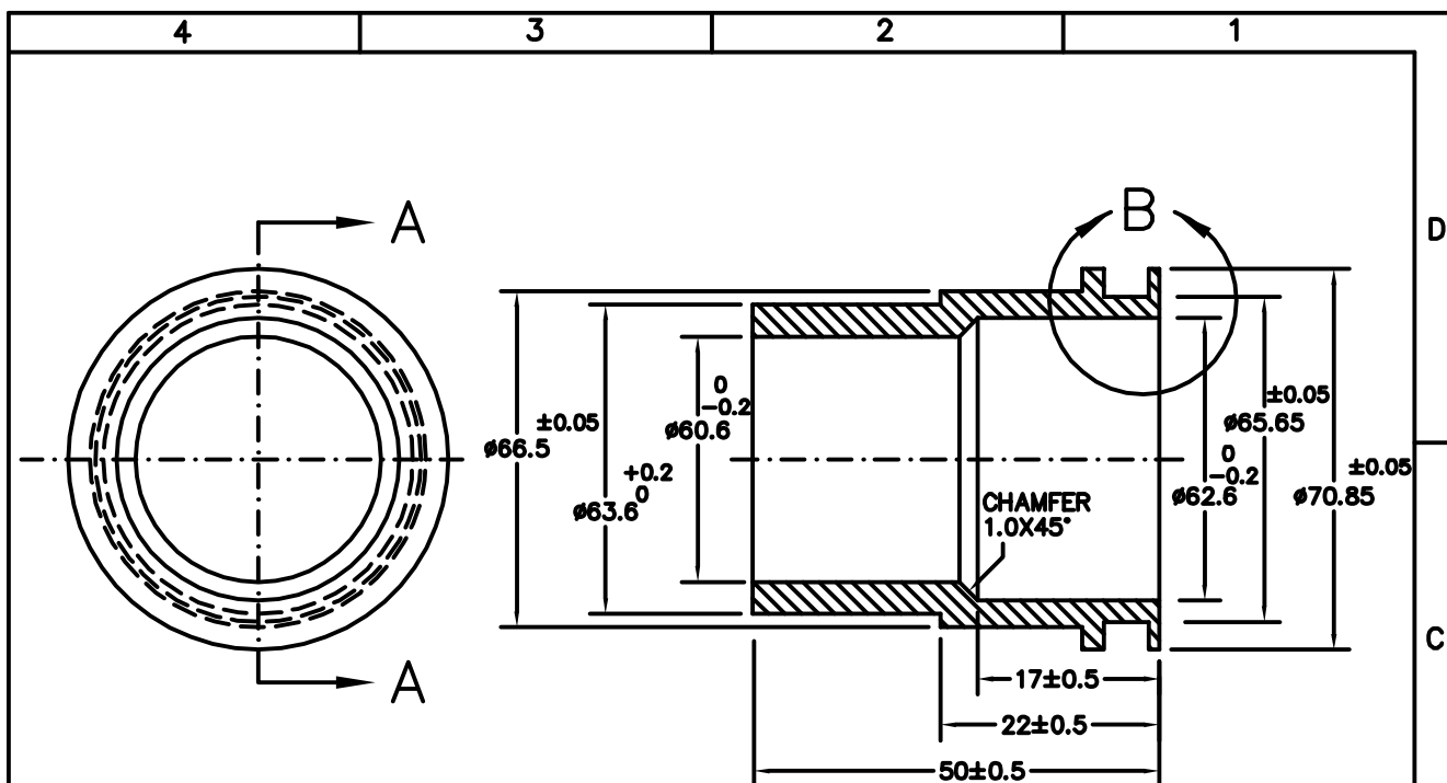
SECTION - AA
