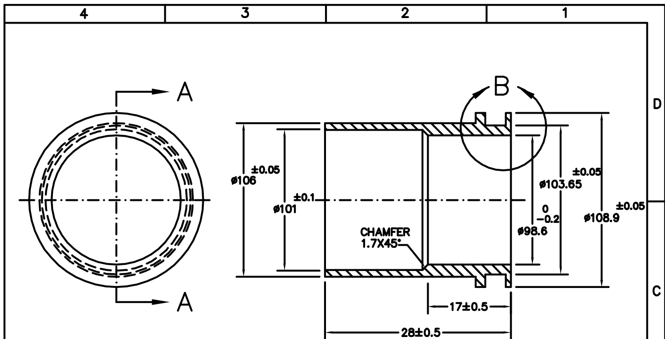
SECTION - AA
