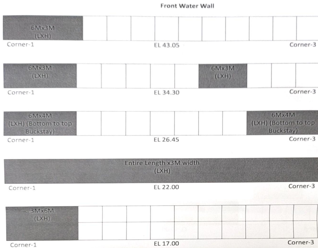
Figure : Front Water Wall
