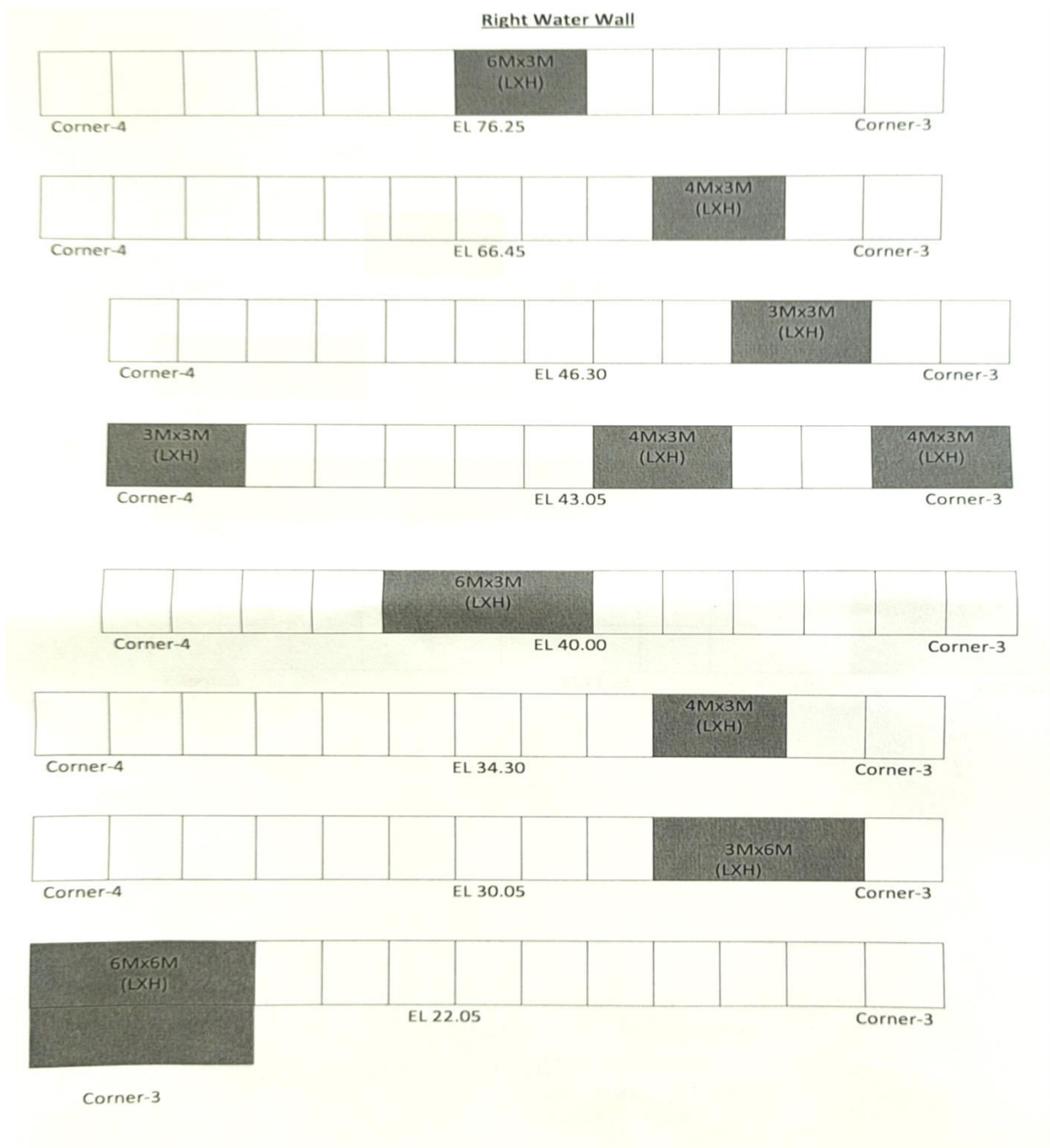
Figure : Right Water Wall
