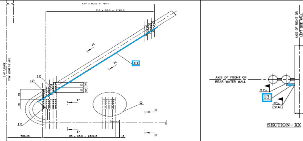
Form work placement in lower transition zone
