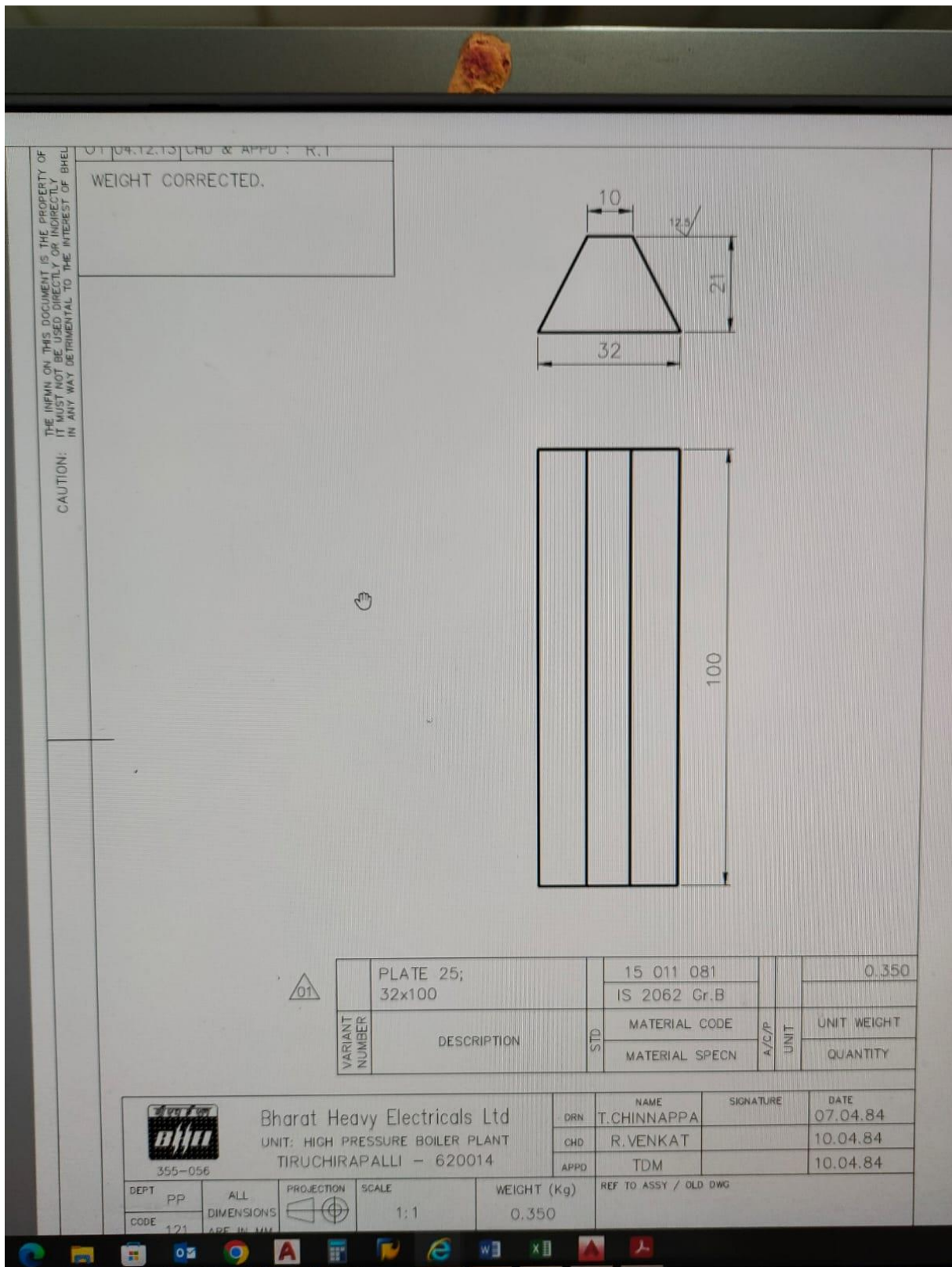
Peg Fin (Trapezium Shaped Bars)
