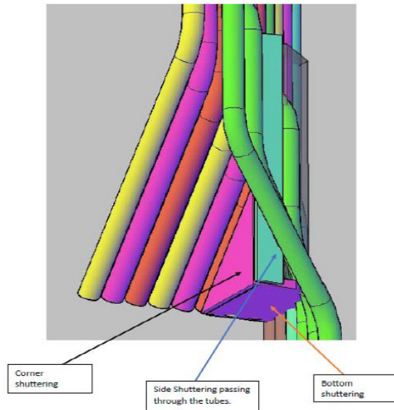
Form work placement in lower transition zone
