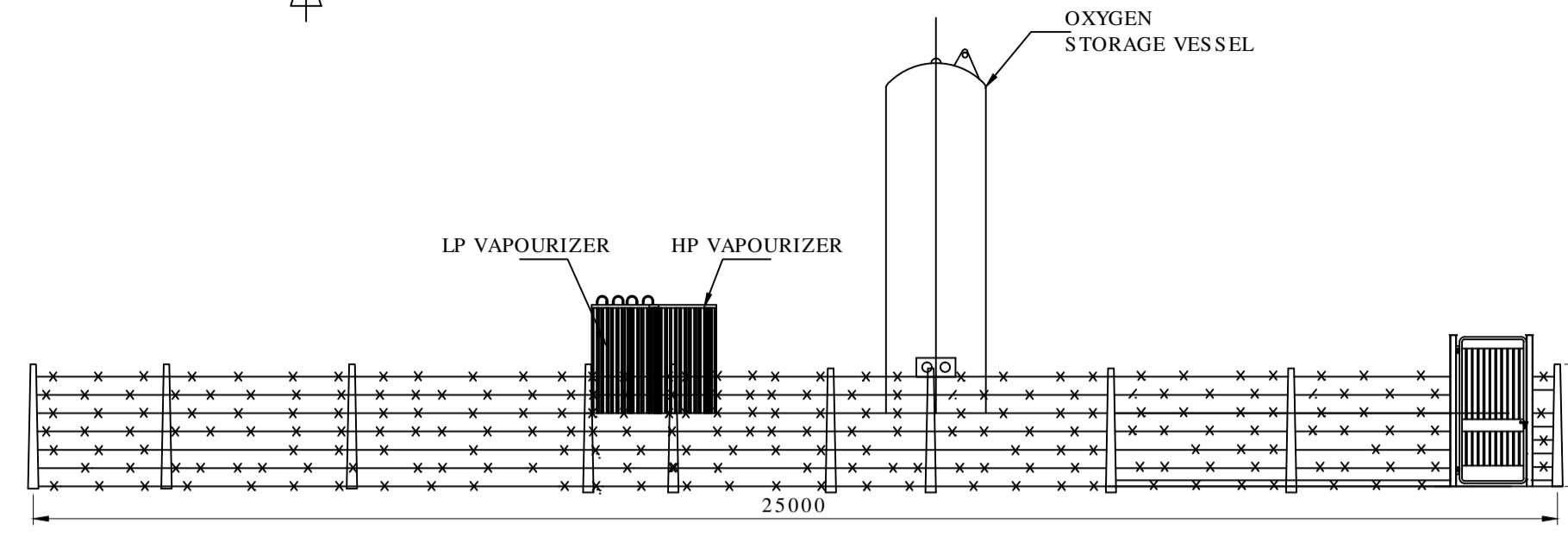
ELEVATION-AA
