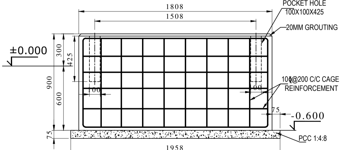
SECTION-YY
