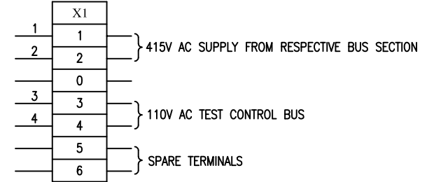
TERMINAL DIAGRAM
