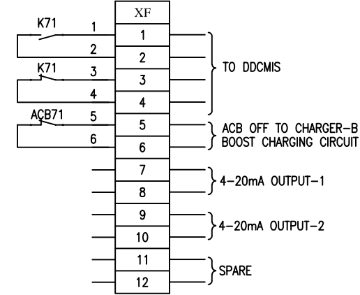
TERMINAL DIAGRAM FROM FLOAT CUM BOOST CHARGER-B
