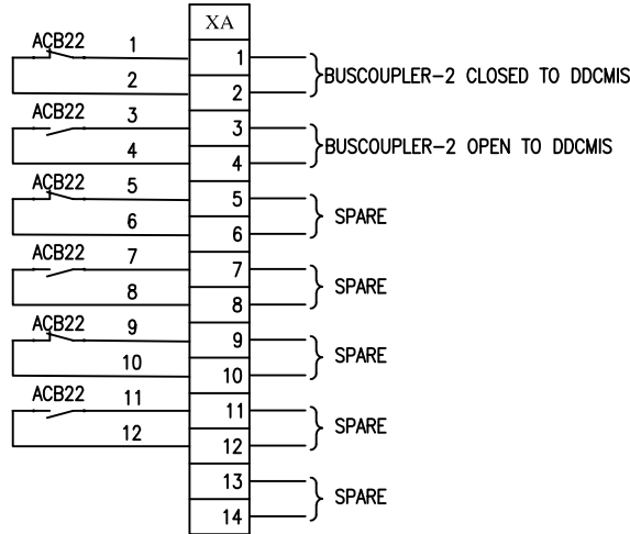
TERMINAL DIAGRAM BUSCOUPLER-2
