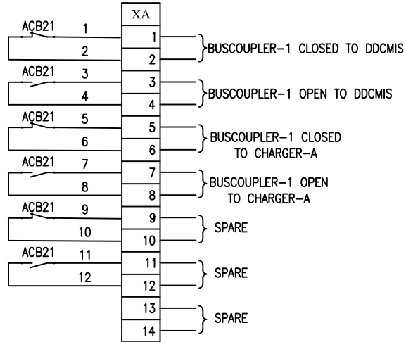
TERMINAL DIAGRAM BUSCOUPLER-1
