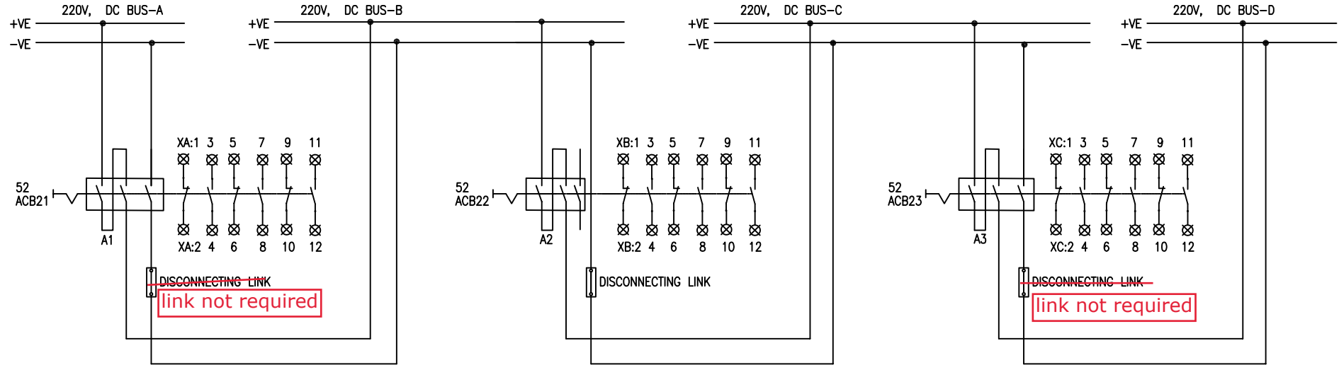
BUSCOUPLER-1
