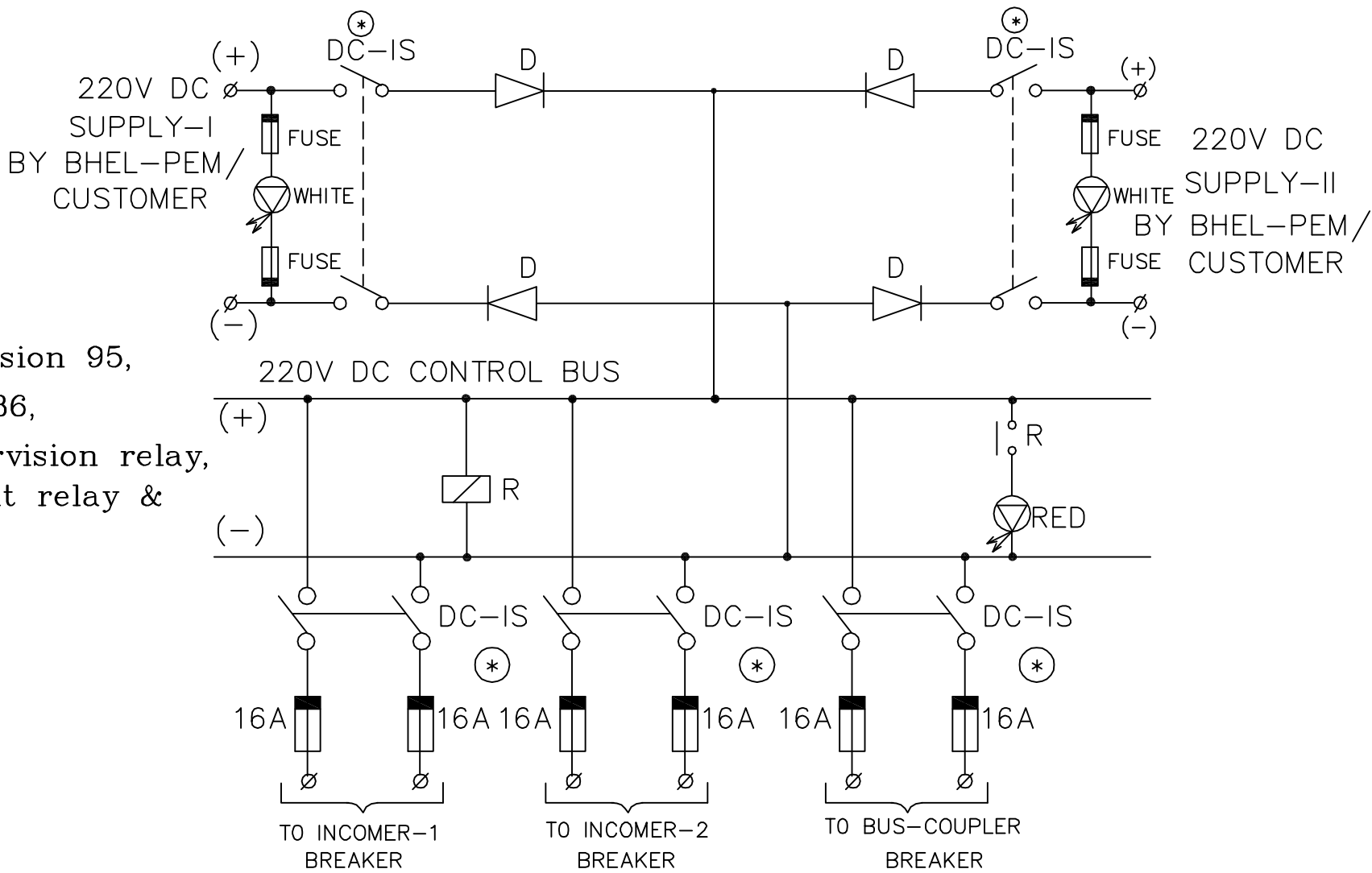
AIR CIRCUIT BREAKER CONTROL SUPPLY CIRCUIT (TYPICAL)
