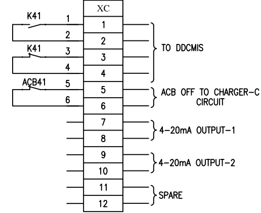
TERMINAL DIAGRAM FROM FLOAT CHARGER-C
