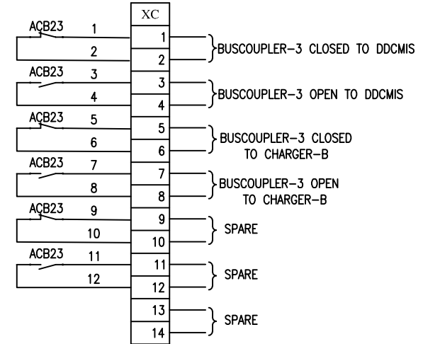
TERMINAL DIAGRAM BUSCOUPLER-3
