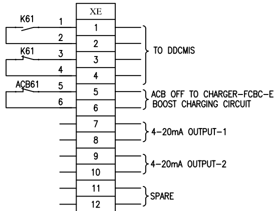
TERMINAL DIAGRAM FROM 220V STANDBY FCBC-E
