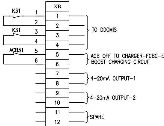
TERMINAL DIAGRAM FROM 220V STANDBY FCBC-E
