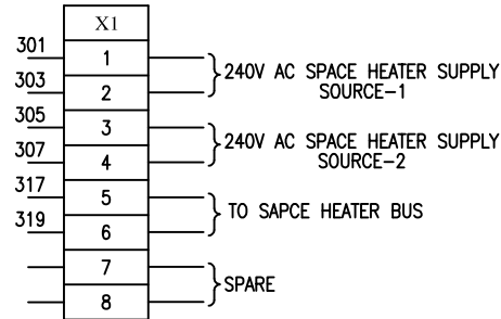
TERMINAL DIAGRAM SPACE HEATER SUPPLY
