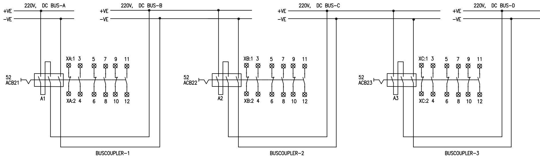
TERMINAL DIAGRAM BUSCOUPLER-1
