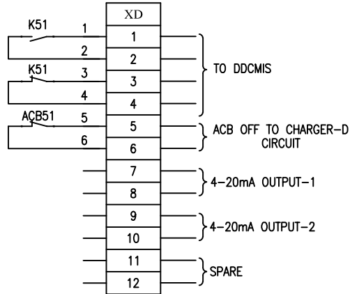
TERMINAL DIAGRAM FROM FLOAT CHARGER-D
