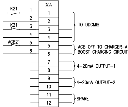
TERMINAL DIAGRAM FROM FLOAT CUM BOOST CHARGER-A
