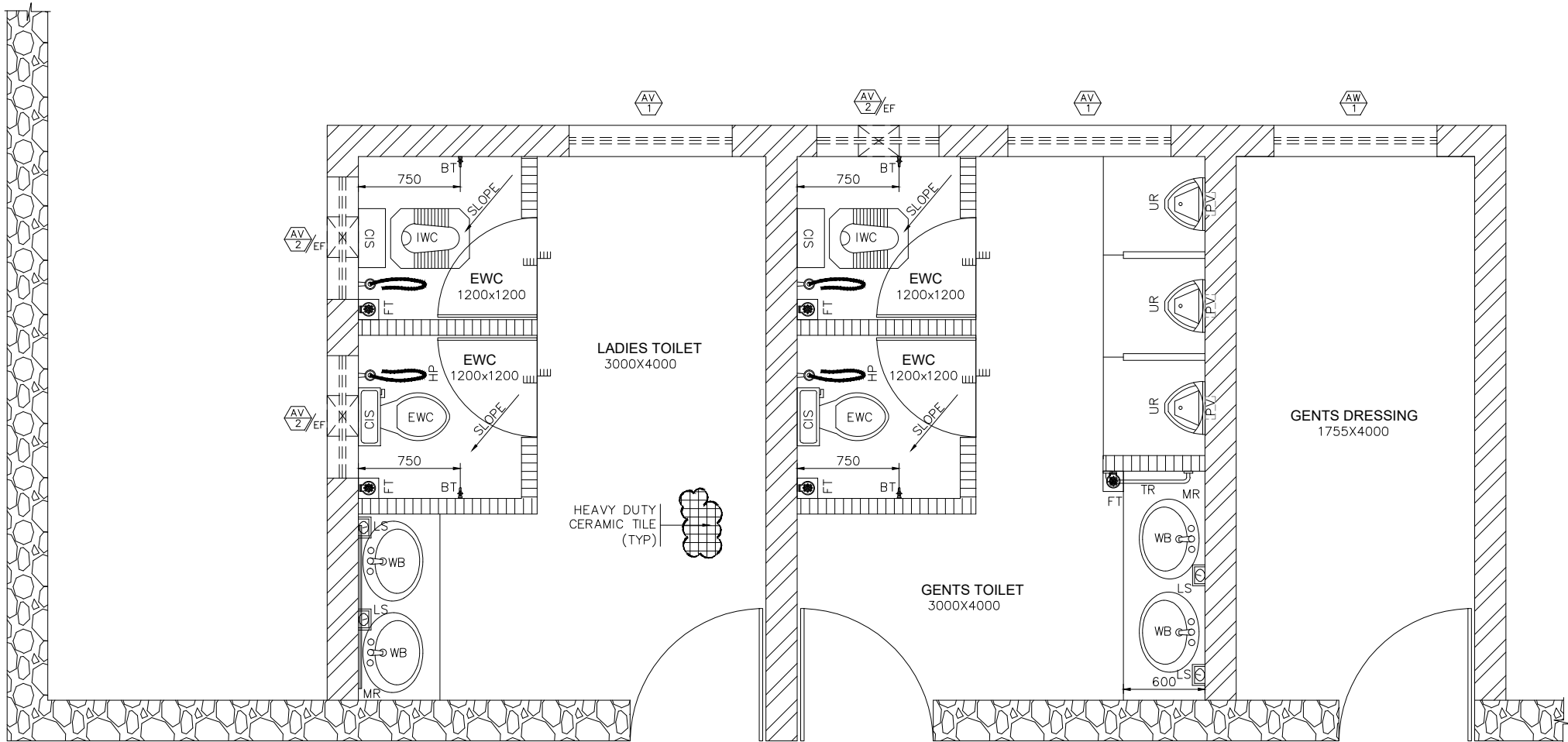
PLAN AT EL(±)0.000M (SCALE 1: 35)
