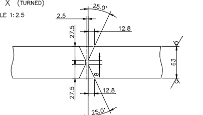
DETAIL X(G4)
