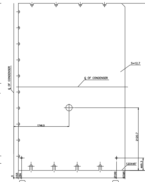
SUPPORT TUBE PLATE 1:2
