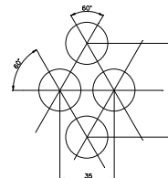
TUBE LAYOUT ARRANGEMENT 10:1
