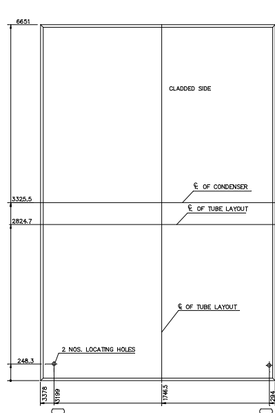
MAIN TUBE PLATE (LS) 1:2
