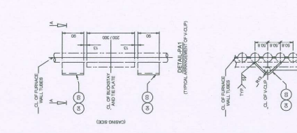
VIEW F ARROW OF ATTACHMENTS ON FURNACE RIGHT SIDE WALL PANEL LOWER (F-18L-7) METALWORKING FROM CHARGE SIDE
