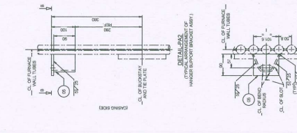
VIEW G ARROW OF ATTACHMENTS ON FURNACE RIGHT SIDE WALL PANEL LOWER (F-18L-7) METALWORKING FROM CHARGE SIDE
