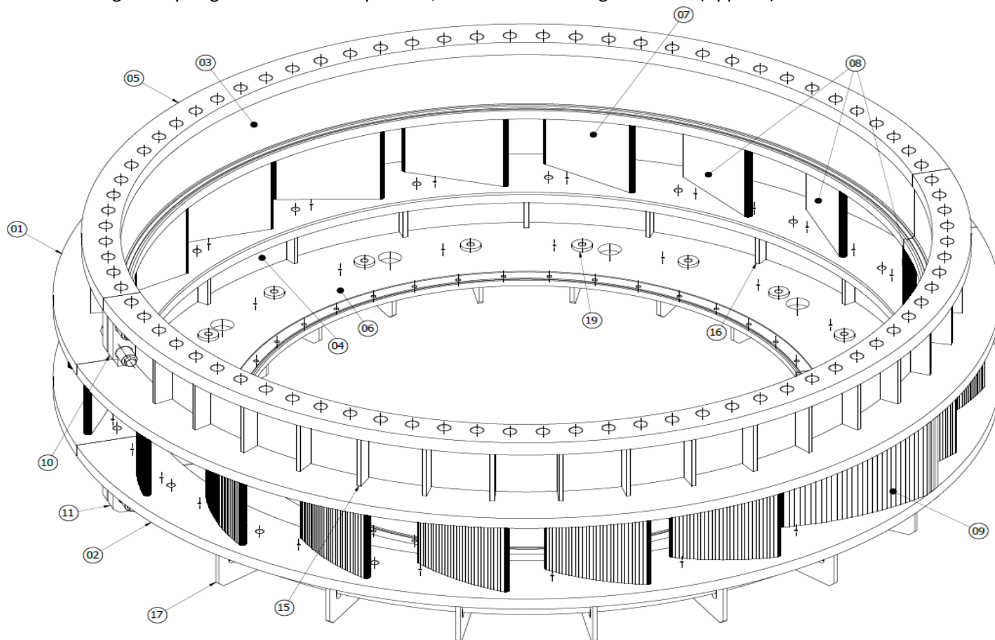
ISOMETRIC VIEW OF STAY RING
