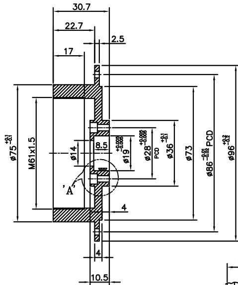
SECTION—'XX'
