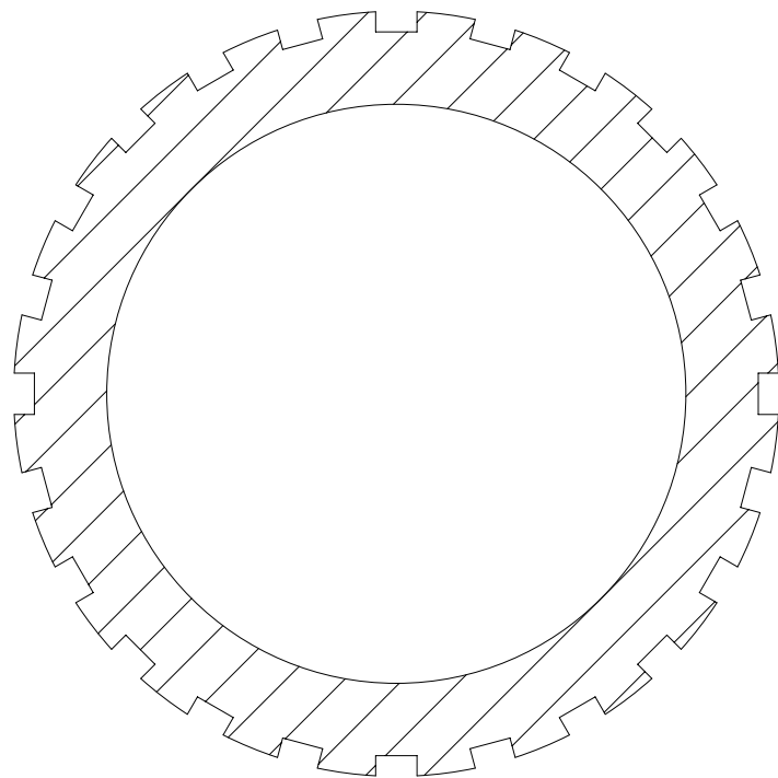
SECTION B-B
