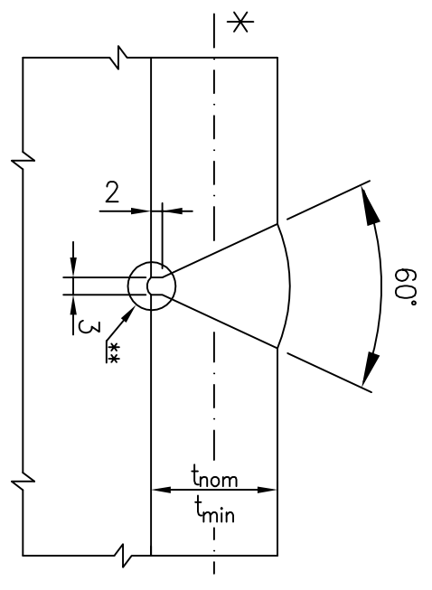
DETAIL - "A"
