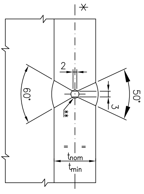
DETAIL - "B"
