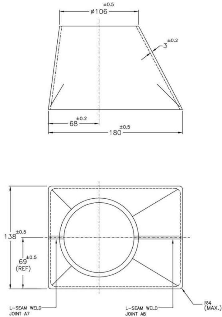
DETAILS OF L-SEAM WELD JOINTS A7,AB
