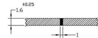
DETAILS OF JOINTS - A7, A8, A9, A10
