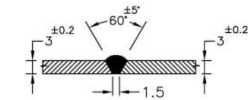
DETAILS OF L-SEAM WELD JOINTS A7,AB
