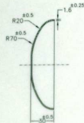
SECTION-BB
