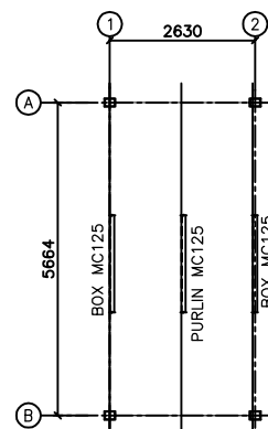
PLAN AT PURLIN LEVEL
