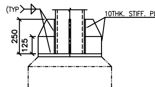
SECTION 1-1
