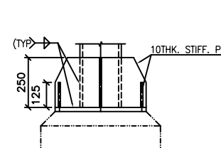
SECTION 2-2
