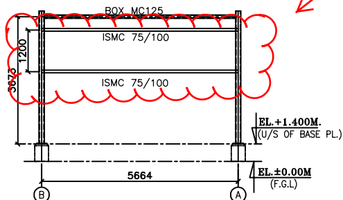
ELEVATION ALONG GRID 1
