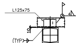
SECTION 3-3
