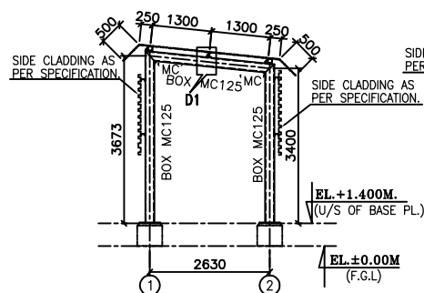
ELEVATION ELEVATION ALONG GRID A
