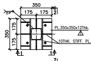
DETAIL OF BASE PLATE (BP-1)
