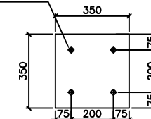
DETAIL OF BASE PLATE
