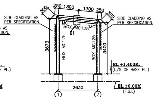
ELEVATION ELEVATION ALONG GRID B
