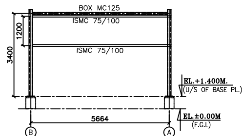
ELEVATION ALONG GRID 2
