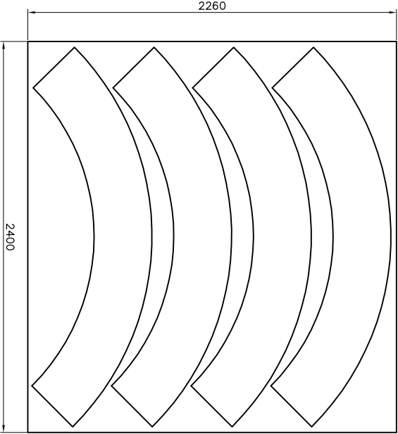
FLANGE CUTTING LAYOUT FOR 10 FLANGE
