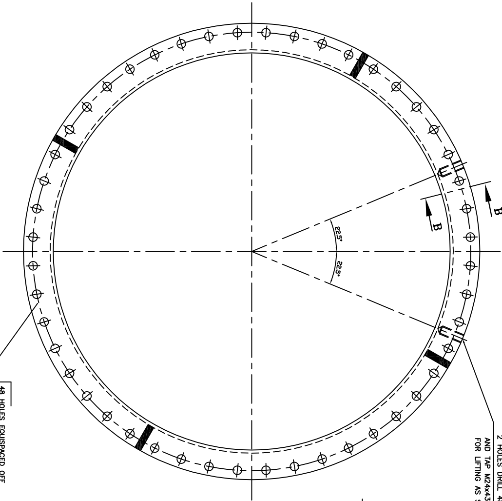
VIEW-C (GRID C-9) (SCALE 1:10)
