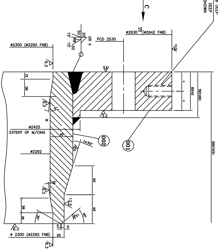
SECTION BB SCALE - 1:2.5 (GRID B-8)
