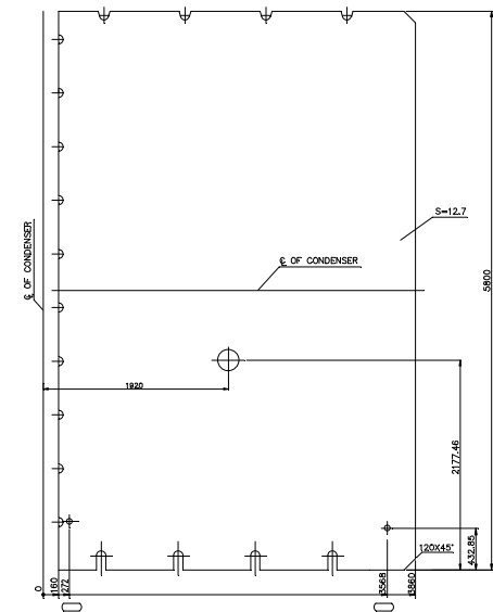
SUPPORT TUBE PLATE 1:2
