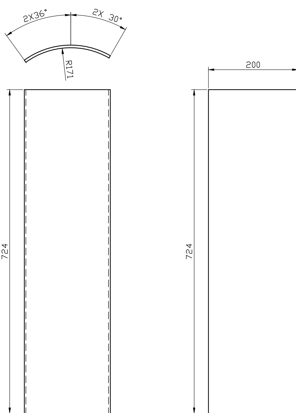
DEVELOPED VIEW
