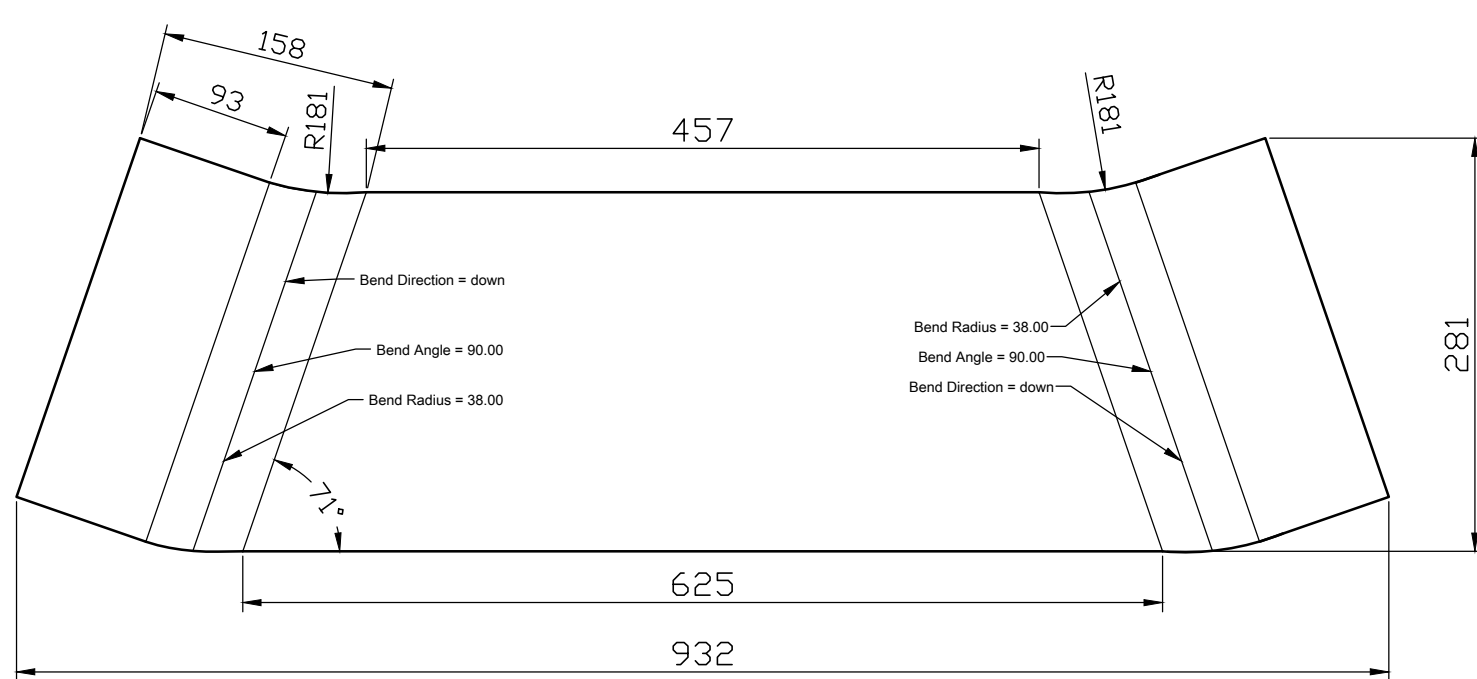
DEVELOPED VIEW (ITEM NO -04)
