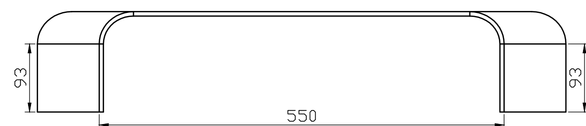
VIEW A
