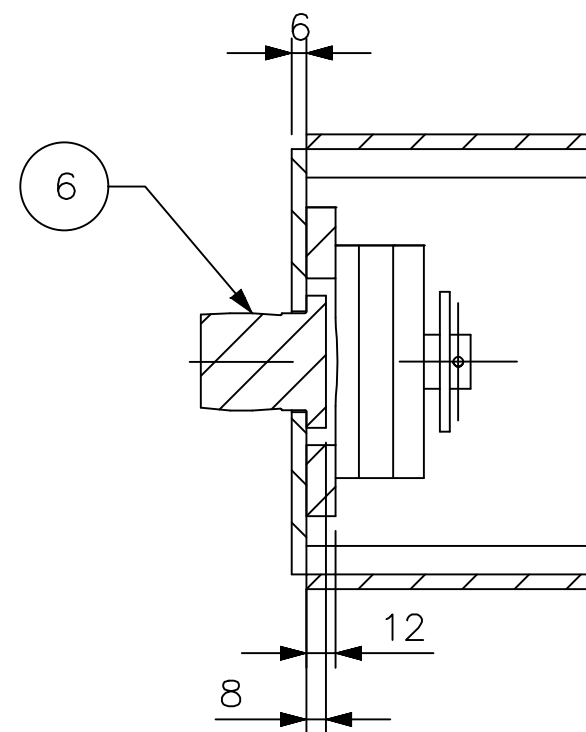
SECTION R-R
