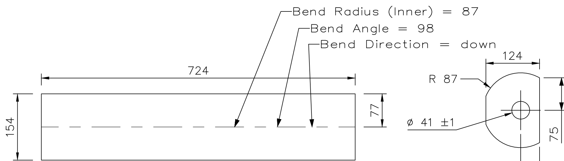
ITEM 1 :: DEVELOPED VIEW
