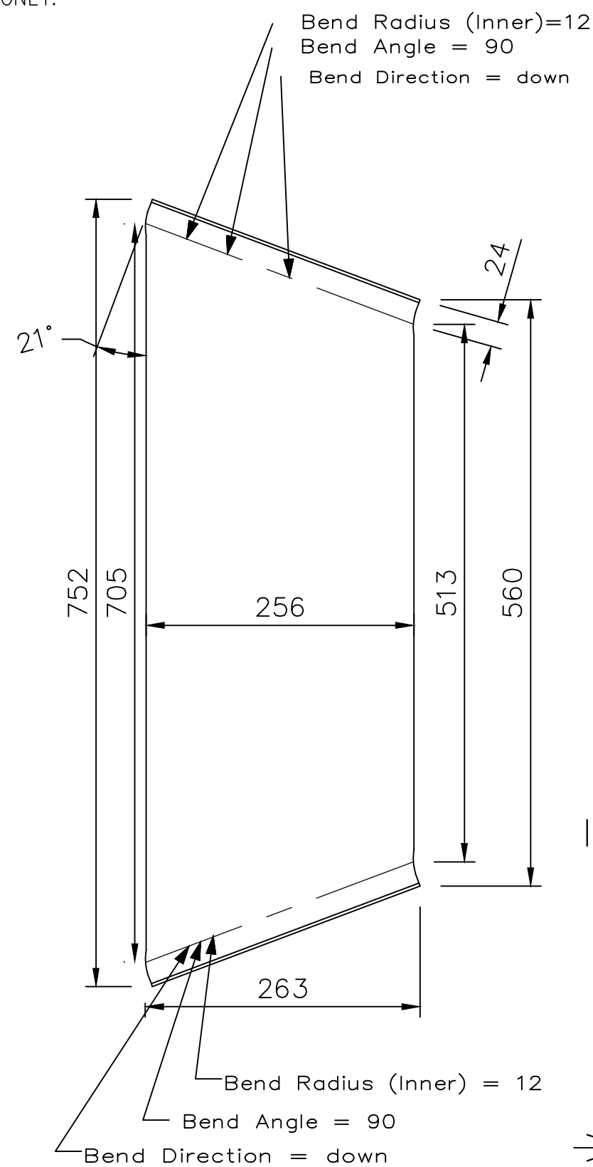
ITEM - 3 DEVELOPED VIEW
