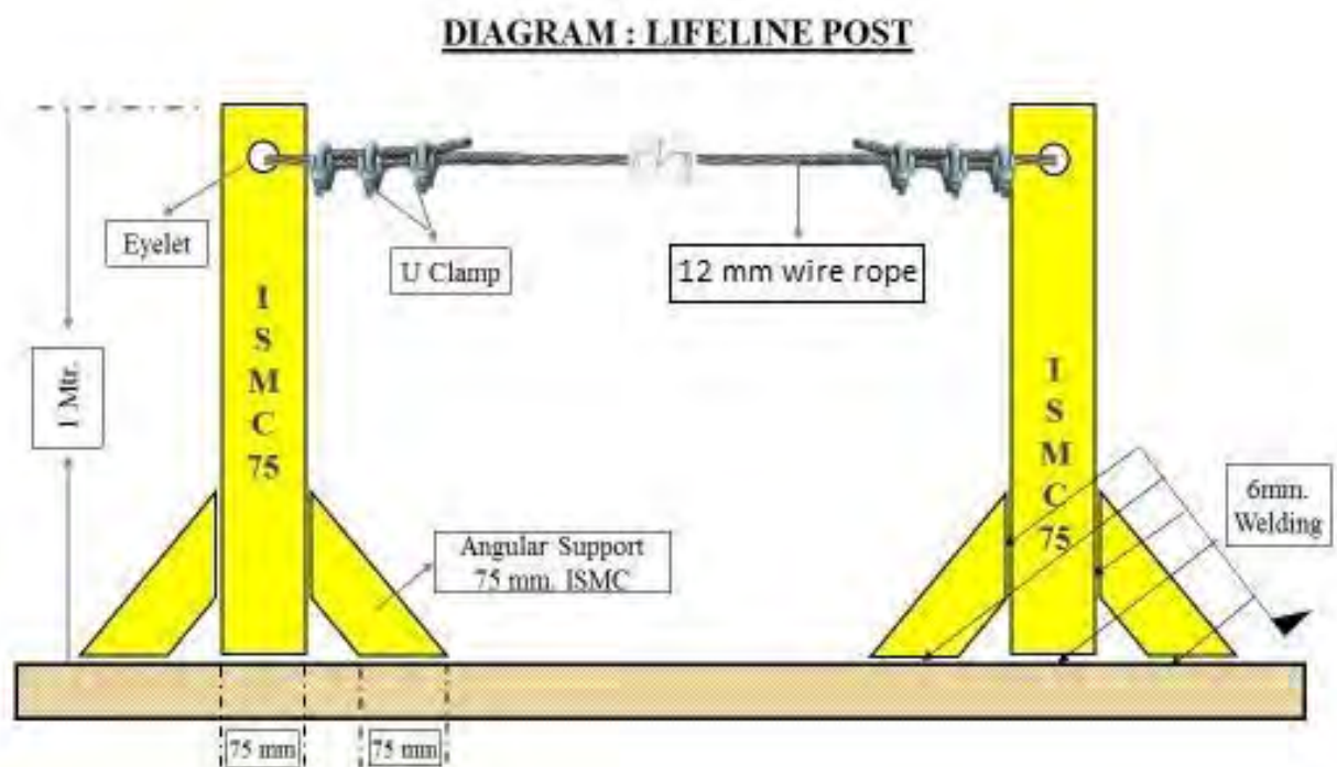
Fig. 2.1 Lifeline Post
