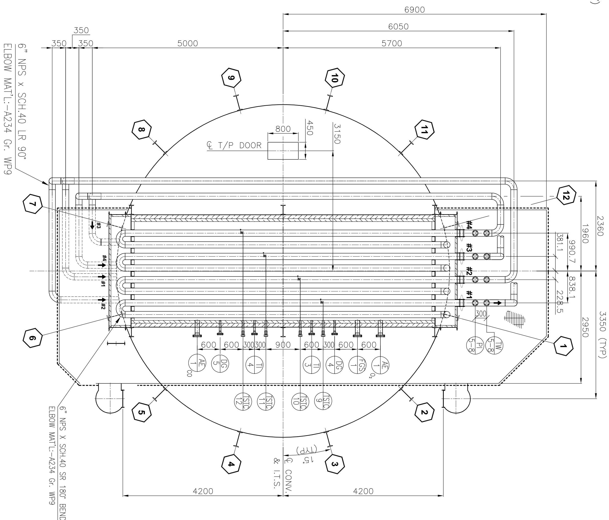
CROSS OVER ARRANGEMENT SECTION F-F
