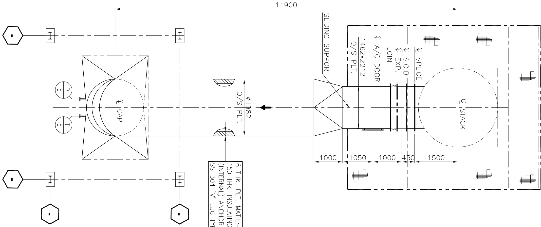
PLAN OF HOT FLUE GAS DUCTING
